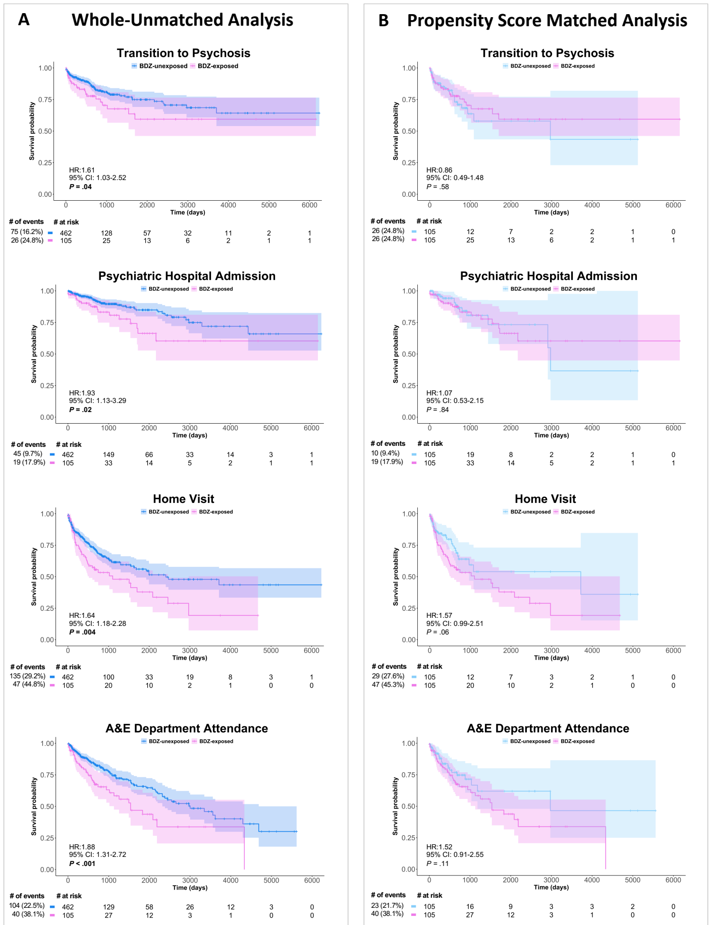
Figure 3. Survival Analysis Comparing the Effect of Benzodiazepine Exposure on the Risk of Subsequent Adverse Clinical Outcomes
