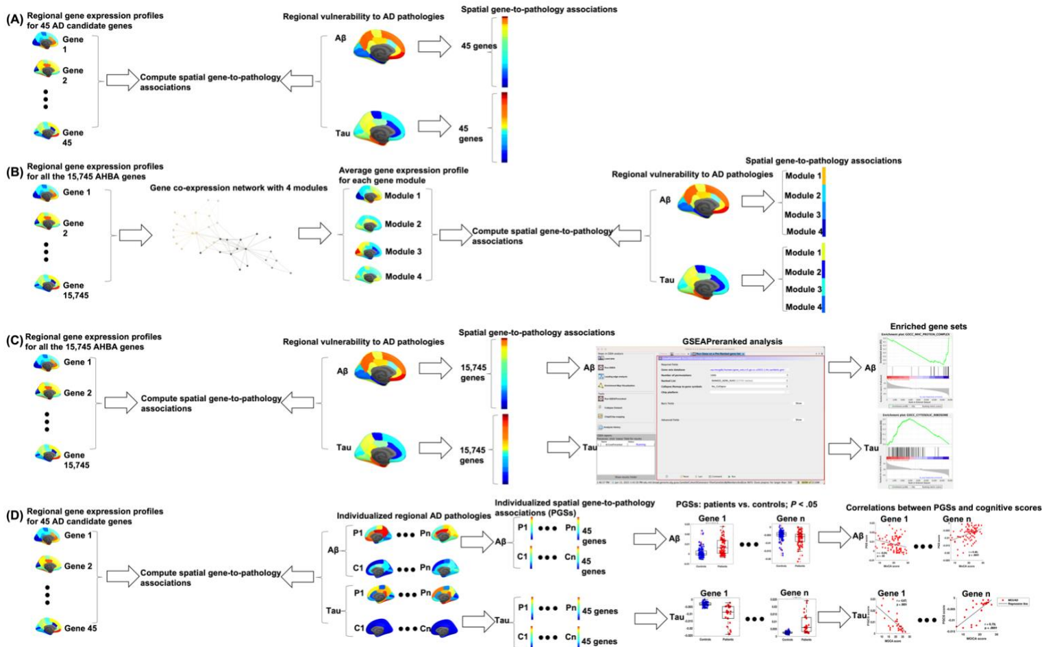
Figure 1. Schematic overview of the applied methods. (A) In a hypothesis-driven analysis, we computed spatial gene-to-pathology associations between brain-wide gene expression profiles of 45 AD susceptibility genes and regional vulnerability to Aβ as well as tau pathologies. We then performed two data-driven analyses (B, C) using regional gene expression profiles of all the 15,745 AHBA genes. (B) We constructed a gene co-expression network, where nodes represent genes and links denote correlations between expression profiles of 15,745 genes. We then identified 4 gene modules and compute spatial associations between average gene expression profiles of the 4 gene modules and regional vulnerability to Aβ as well as tau pathologies. (C) We computed spatial associations between brain-wide gene expression profiles of 15,745 genes and regional vulnerability to Aβ as well as tau pathologies. We then used the GSEA software to conduct GSEAPreranked analysis on the ranked spatial correlations and identified enriched gene sets. (D) We computed personalized spatial gene-to-pathology associations between brain-wide gene expression profiles of 45 AD susceptibility genes and individualized regional Aβ and tau pathologies, resulting in individual-level Aβ- and tau-related pathogenetic scores (PGSs). Then, we estimated group differences of PGSs between patients (MCI and AD) and controls (CU and/or SCD) for each gene. Finally, for the genes showing significantly different PGSs between groups, we computed Pearson’s correlations between the PGSs and cognitive scores (e.g., MoCA and MMSE). The above analyses (A-D) were performed using both the ADNI (discovery) and IMAS (replication) datasets. Analysis (D) was also performed using average expression profiles of 4 gene modules identified in analysis (B) . Abbreviations: CU = cognitively unimpaired; SCD = subjective cognitive decline; MCI = mild cognitive impairment; AD = Alzheimer’s disease; IMAS = Indiana Memory and Aging Study; ADNI = Alzheimer’s Disease Neuroimaging Initiative; MoCA = Montreal Cognitive Assessment; MMSE = Mini-Mental State Exam; GSEA = gene set enrichment analysis.
