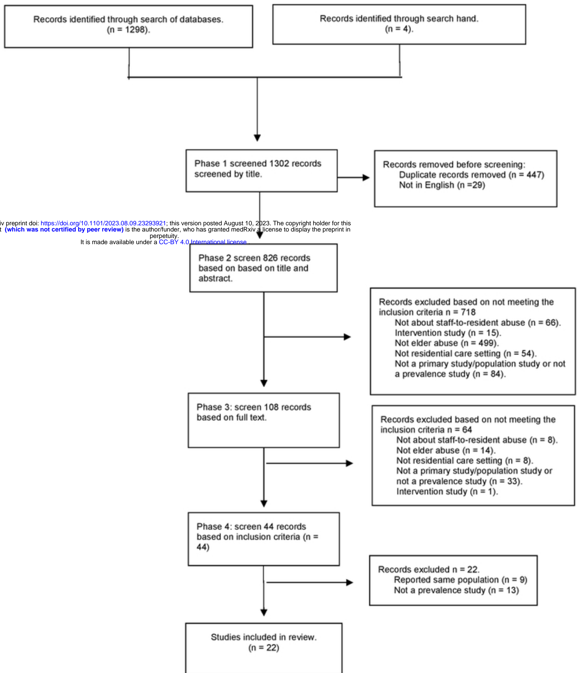
Fig. 1. Identification and Selection of Studies – PRISMA flow diagram [14]
