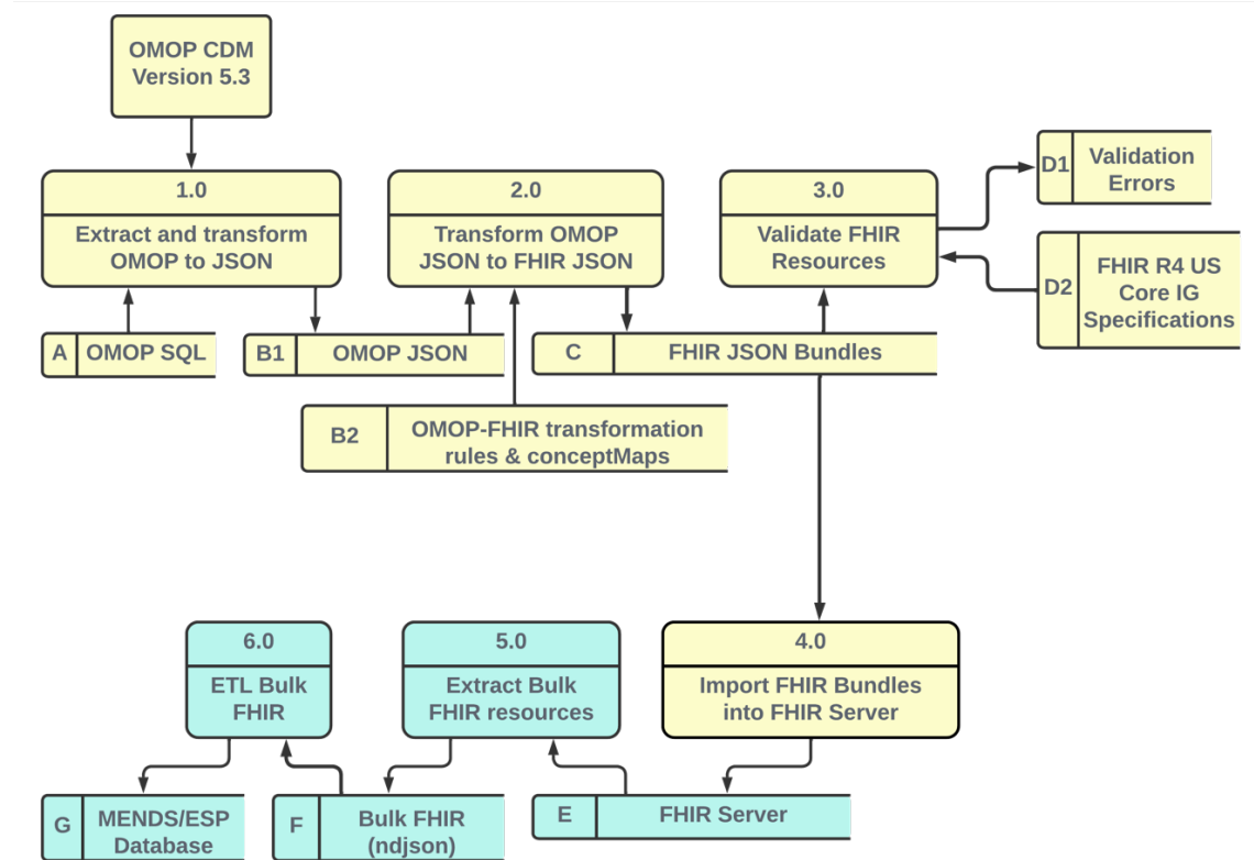
Figure 1. Level 1 logical data flow diagram. Yellow components perform the OMOP-to-FHIR transformation and FHIR server upload. Green components perform the Bulk FHIR export and FHIR-based ETL into the MENDS database.
