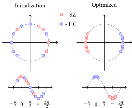
Figure 3. Normalization of data points inside the unit circle, using layer normalization, along with the optimization of a contrastive loss lead to correct separation of sinusoids. Data points belong to two classes, HC and SZ , that are separated after the minimization of \mathcal{L}_D . Because we separate false pairs, according to (1 - y_p) \times \|D(x_1, x_2) - m\|_1 , all points are placed within a shift variant interval of the cosine. The variance needed for classification.
