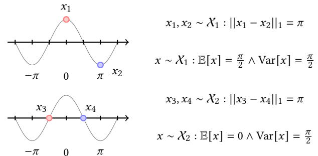
Figure 2. Description of how two similarly distributed samples, taken from \mathcal{X}_1 and \mathcal{X}_2 , can lead to different portions of the cosine function image, since a sinusoid is periodic. Two distributions \mathcal{X}_1 and \mathcal{X}_2 , may be mapped to the same image (second/bottom example). This is why a cosine is a shift invariant function. However, there are intervals a shift can be made and it is not invariant. Such intervals take the form \forall i \in \mathbb{Z} : [i\pi, (i+1)\pi] .
