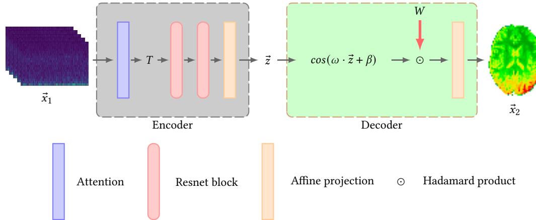
Figure 1. The neural architecture has two components: an Encoder (shaded in grey) and a Decoder (shaded in green). The input is the stft v_1 representation. The output is the synthesized fmri . The Encoder begins with a simple attention mechanism on the channels dimension of the stft . After, it is processed by two Resnet blocks and an affine layer. This produces the latent representation \tilde{z} . Following, comes the Decoder, which picks this representation and builds the cosine bases through the projection \omega \cdot \tilde{z} + \beta . The sinusoids are style induced with \cos(\omega \cdot \tilde{z} + \beta) \odot W . The vector W is a style fixed pretrained vector of an fmri representation, learned from a simultaneous EEG and fMRI dataset (described in Section 3.1). Finally, an affine layer projects it to the fmri space.
