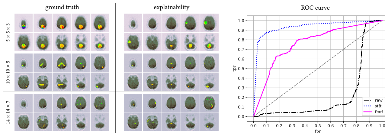
Figure 5. We analyzed resolutions \in \{5 \times 5 \times 3, 10 \times 10 \times 5, 14 \times 14 \times 7\} and gathered the biclusters retrieved for the ground truth and predicted labels. Only the best biclusters (with the best lift ) are shown in this figure for each setting. On the right side, the receiver operating characteristic (ROC) curve is shown. The raw view performed below random, while the stft and fmri were above. The stft is close to a perfect classifier.
