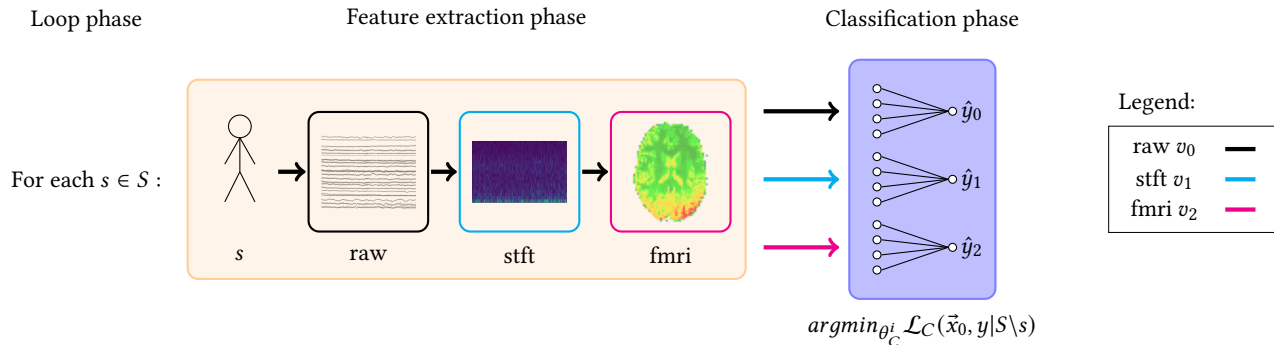
Figure 4. We do a leave-one-individual-out validation, where for each fold we either train a linear classifier with raw , stft or fmri representations. Each representation has its own validation. The arrows inside the feature extraction phase indicate dependency, that is: an fmri representation needs a stft ; stft needs the raw ; and the raw , of course, needs an individual’s recording, denoted with a human figure. For each fold, s \in S , we train a linear classifier without s , \arg\min_{\theta_C} \mathcal{L}_C(\hat{x}_0, y | S \setminus s) . In addition, the fmri setting also optimizes \arg\min_{\theta_E} \mathcal{L}_D . For all individuals/folds the predictions are saved to compute the are under the curve (AUC) against the ground truth.
