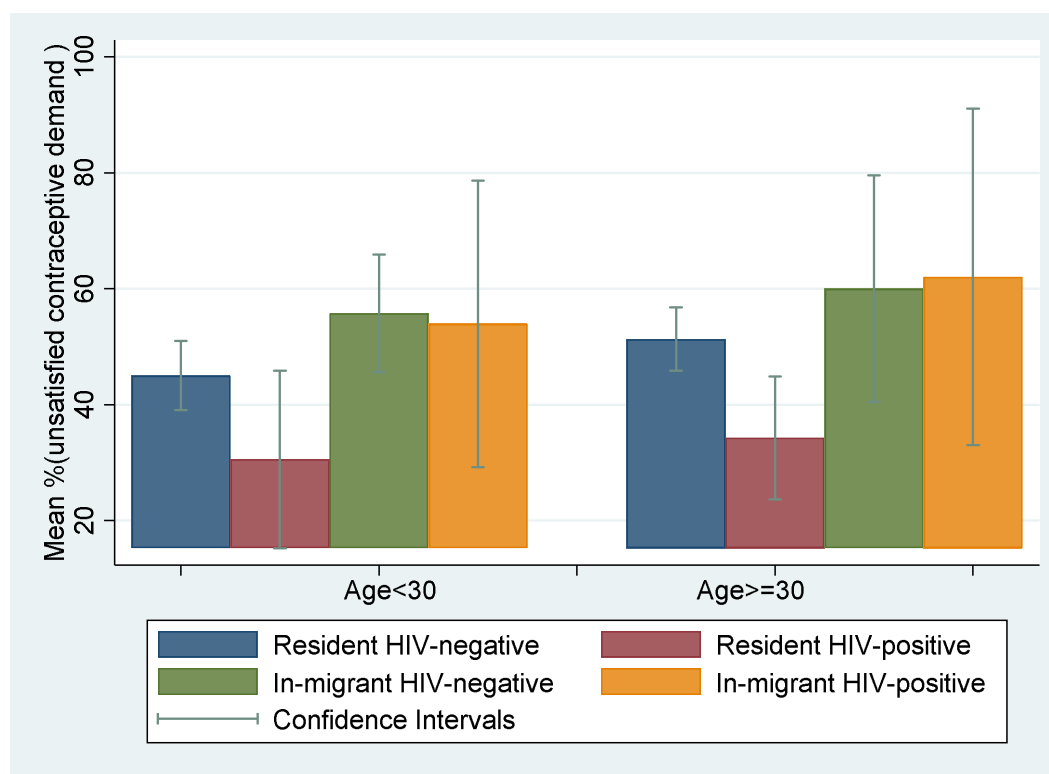
Figure 1. Prevalence of unsatisfied contraceptive demand by recent migration history and HIV serostatus stratified by age among 3,417 sexually active females with no intention of getting pregnant in the next year.
