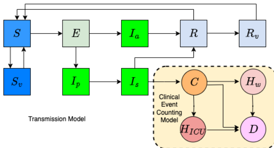
Fig. 1 Schematic of the transmission process, and clinical event counting model.
