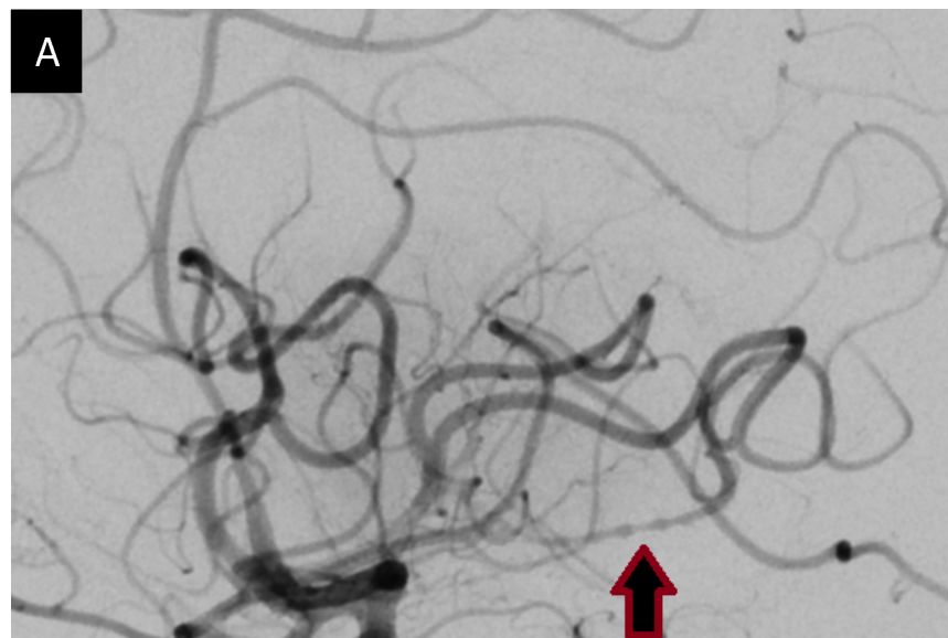
Figure 2 – (A) Medium-vessel vasospasm in the left middle cerebral artery proximal M3-segment during endovascular stroke treatment (EVT); (B) study group comparison response on treatment of the vasospasm
