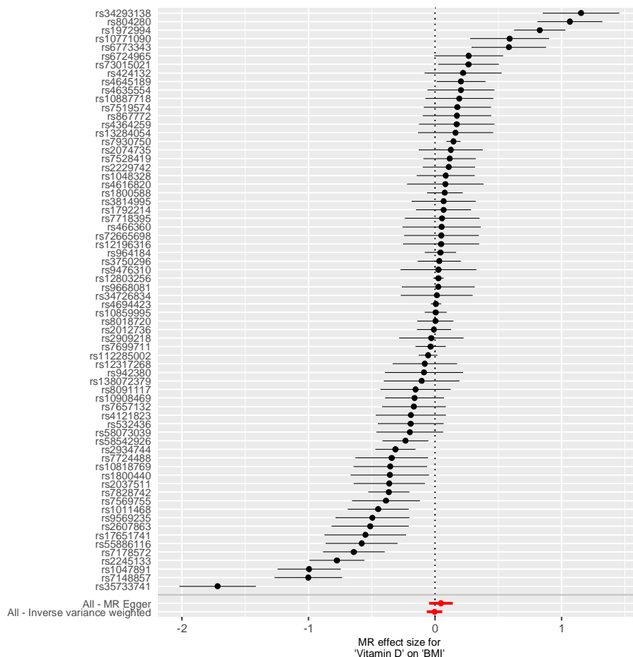
Figure 2: Forest plot of the results from the single SNP Wald estimation
