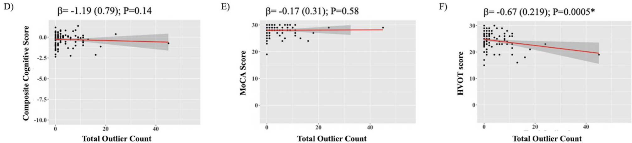
Figure 3. Relationship between total outlier count and cognitive measures in DLB and PD. Regression plots for the association between total outlier count (independent variable) and the following dependent variables: Composite Cognitive score, MoCA and Hooper Visual Organisation Test, in DLB (A, B, C, respectively) and PD (D, E, F, respectively). \beta coefficient values, corrected for age and sex, are presented along with P values. * denotes significant association.
