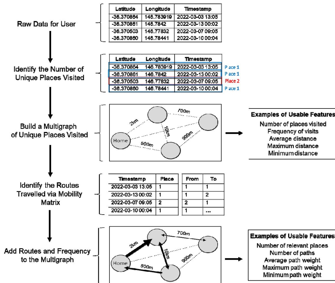
Figure 1. Schematic of the steps used to process raw passive sensing data collected from users' mobile phones and identify usable features for subsequent statistical analyses and predictive modelling.
