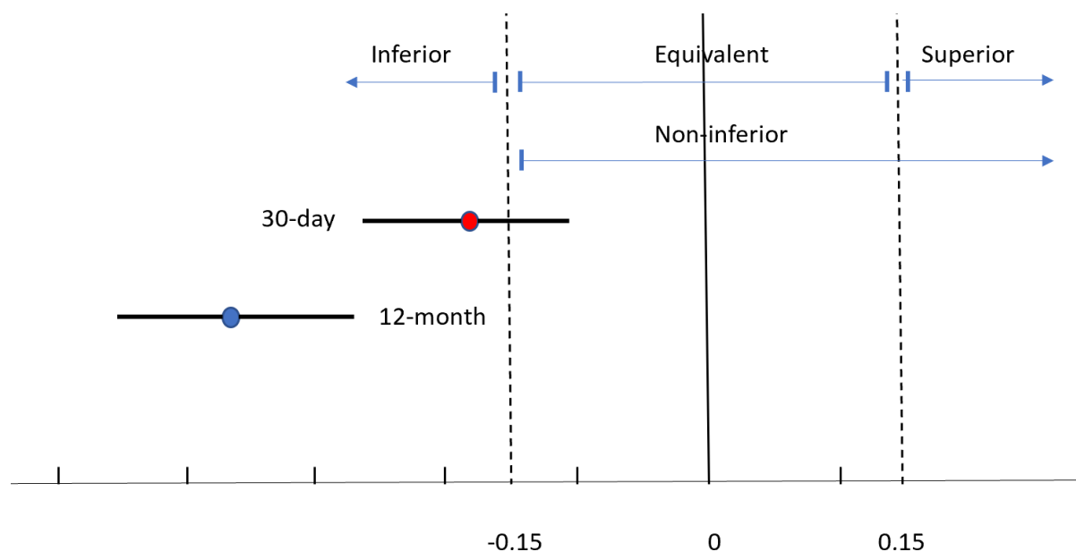
Figure 3: Treatment success proportional difference between operative management (OM) and non-operative management (NOM).
