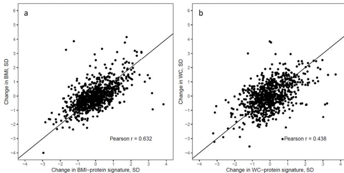
663 664 Supplementary Figure 2. Scatterplots of (a) change in BMI against change in BMI-protein signature, 665 and (b) change in WC against change in WC-protein signature over a ~6-year period in the T2DCC 666 set. The diagonal lines represent the y = x line. Abbreviations: BMI, body mass index; SD, standard 667 deviation; T2DCC, type 2 diabetes case control; WC, waist circumference.
