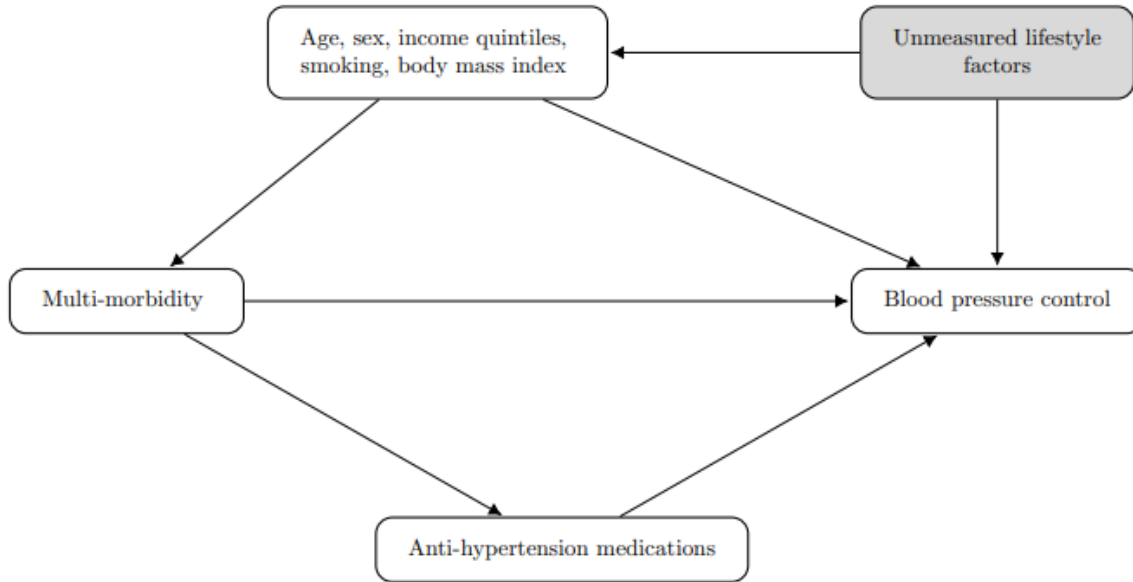
430 Figure S1: Directed acyclic graph for the effect of multi-morbidity on blood pressure control
