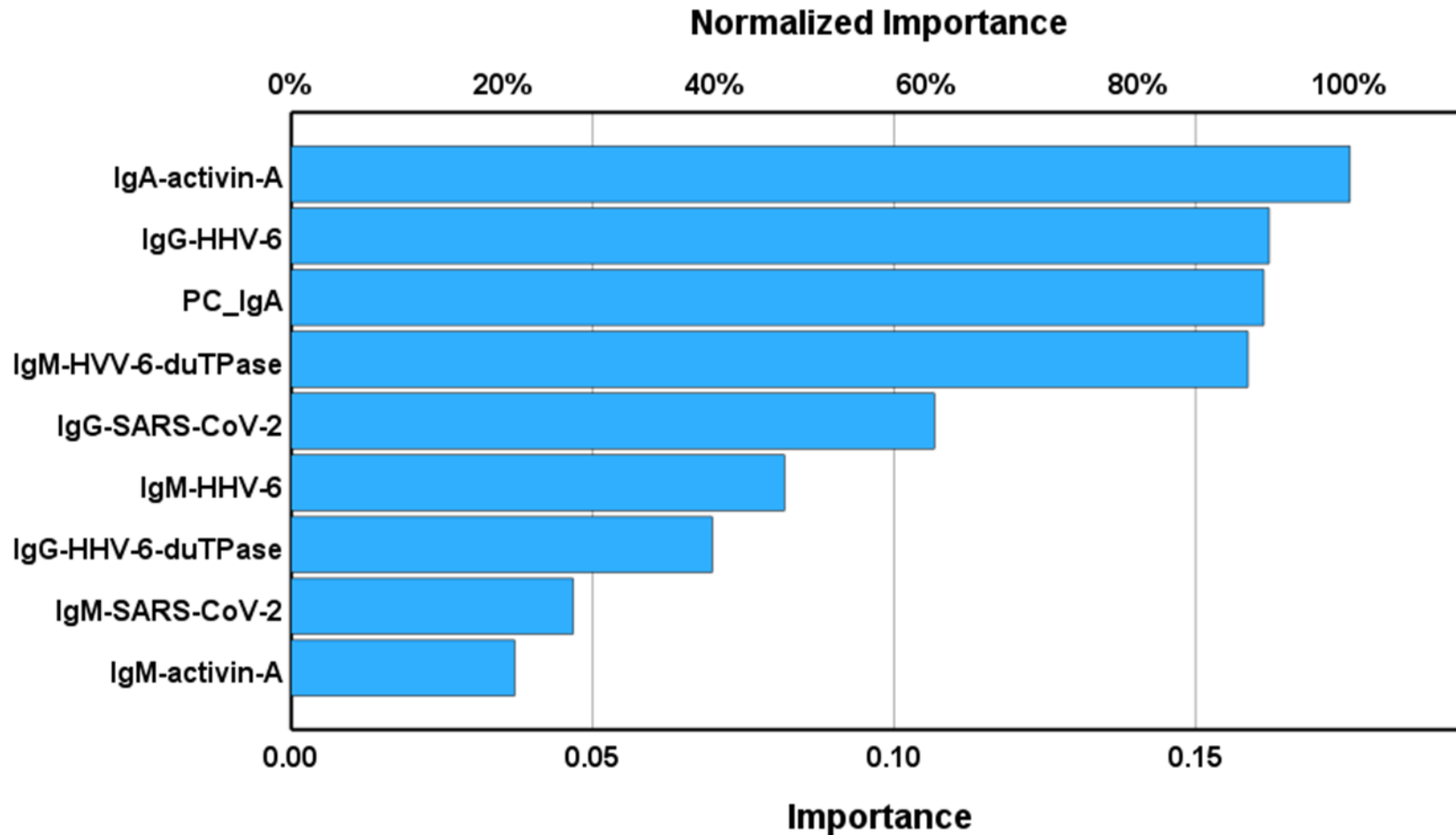
Figure 2. Importance chart of a neural network analysis with Long COVID patients versus controls as output variables. Ig: Immunoglobulin. HHV: Human Herpes Virus, duTPase: deoxyuridine 5'-triphosphate nucleotidohydrolase, SARS-CoV-2: severe acute respiratory syndrome coronavirus 2, PC_IgA: principal component extracted from all IgA values against viral antigens.
