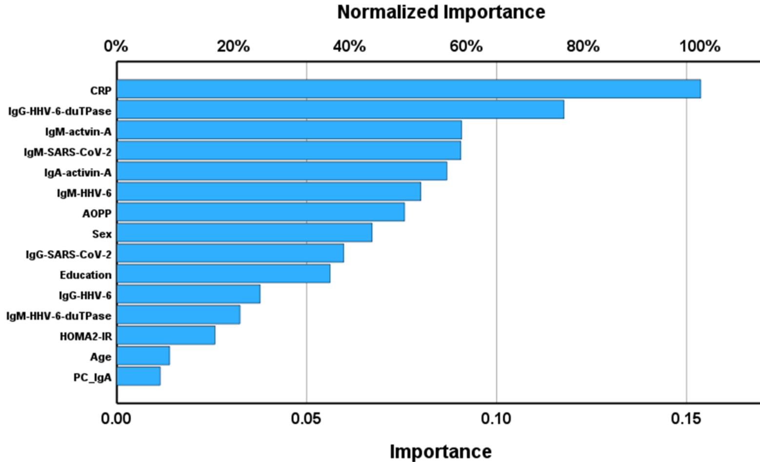
Figure 4. Importance chart of neural network analysis with to total Fatigue-Fibromyalgia (FF) score as dependent variable. Ig: Immunoglobulin. HHV: Human Herpes Virus, duTPase: deoxyuridine 5'-triphosphate nucleotidohydrolase, SARS-CoV-2: severe acute respiratory syndrome coronavirus 2, PC_IgA: principal component extracted from all IgA values against viral antigens, AOPP: advanced oxidation protein products, CRP: C-reactive protein, HOMA2-IR: Homeostatic Model Assessment for Insulin Resistance.
