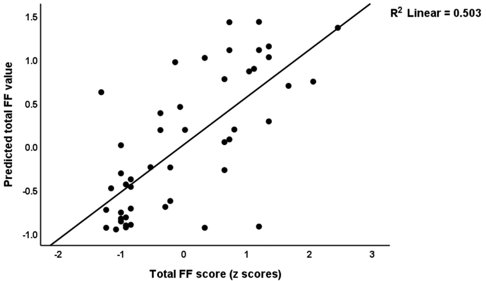
Figure 5. Predictive accuracy of the neuronal network (NN#3) shown in Figure 4 and Table 3; the predicted versus observed value of the Fibro-Fatigue score.
