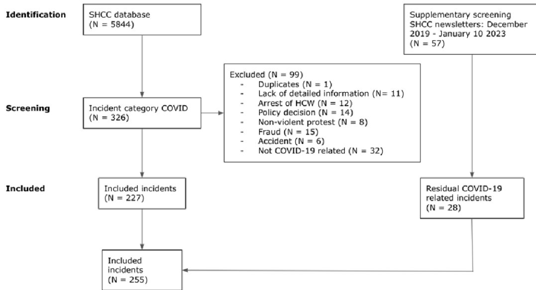
Fig 1. PRISMA flowchart
