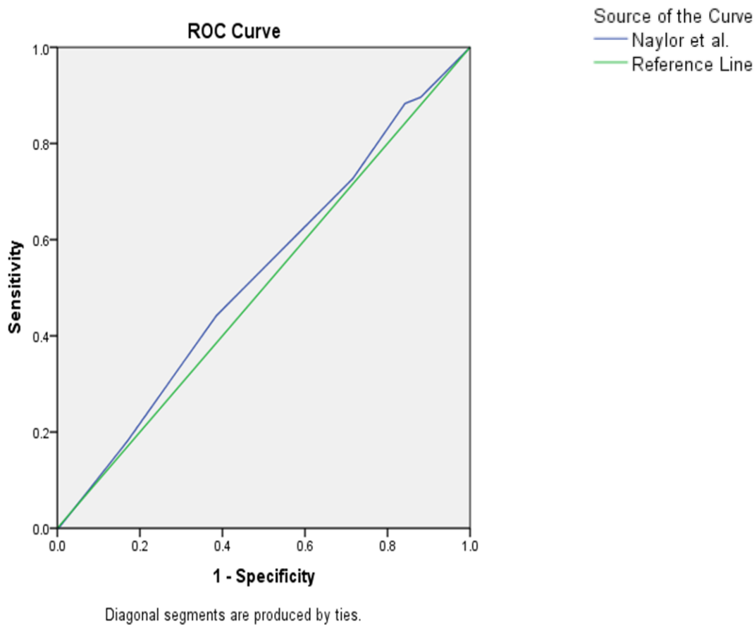
Figure 1: Receiver operating characteristic curves showing performance of Naylor et al clinical risk score in predicting GDM.
