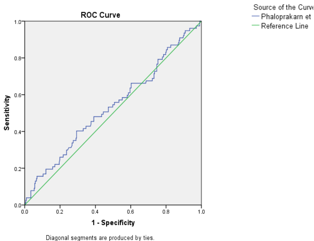
Figure 3: Receiver operating characteristic curves showing performance of Phaloprakarn et al clinical risk score in predicting GDM.
