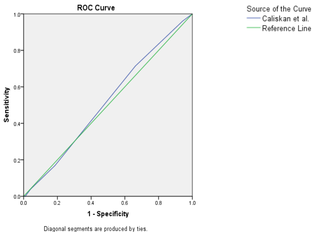
Figure 2: Receiver operating characteristic curves showing performance of Caliskan et al clinical risk score in predicting GDM.
