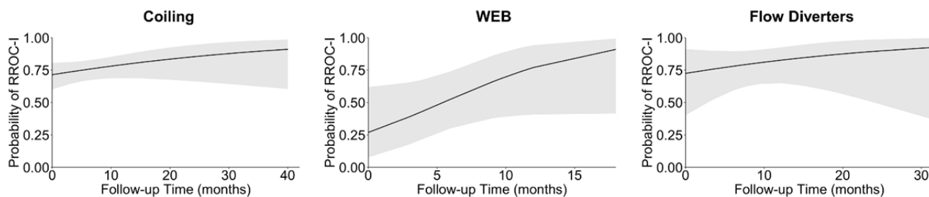
198 Figure 2. LGLMM model fits for probability of RROC-I as a function of follow-up time for the 199 evaluated endovascular therapy techniques. Grey shading represents CI 95%. 200
