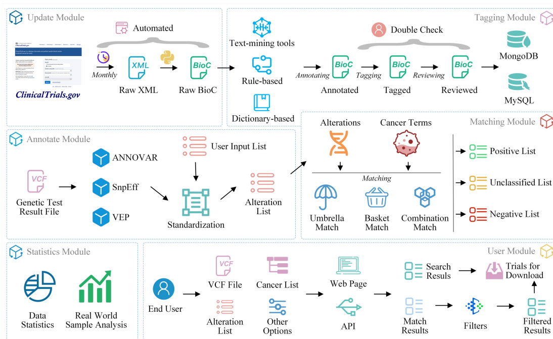
Figure 1. An overview of OncoCTMiner modules.
