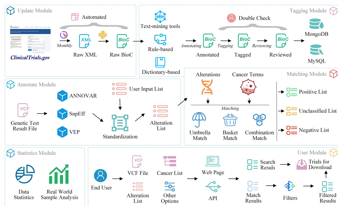
Figure 1. An overview of OncoCTMiner modules.
