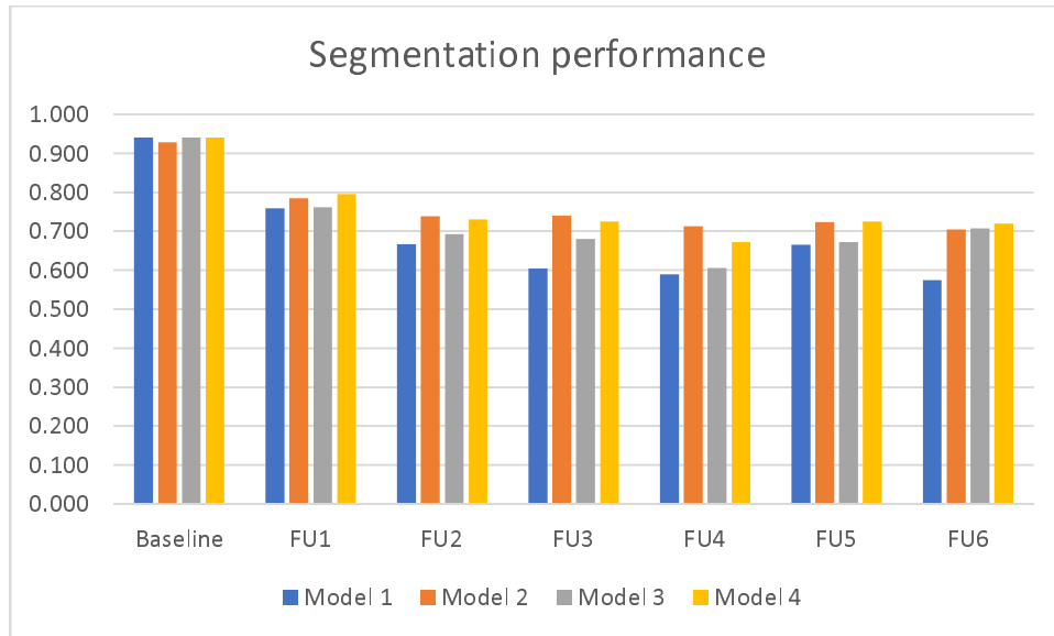
Figure 1: DSC of the segmentation models
