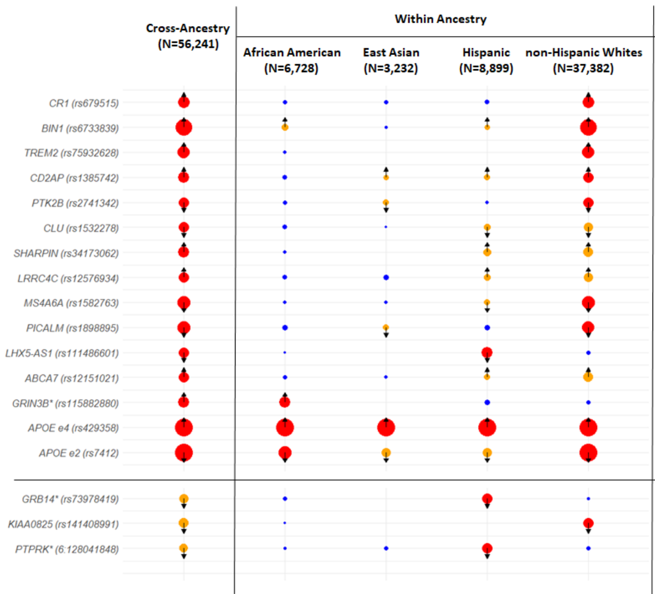
Figure 2. Ancestry comparison plot of the multi-ancestry GWAS associations. The plot displays results for 18 loci associated with AD risk within and across multiple ancestries. Circle size corresponds to the significance level, -\log_{10}(P\text{-value}) , and circle color represents the significance threshold: red, P < 5 \times 10^{-8} ; orange, 0.05 > P > 5 \times 10^{-8} ; and blue, P > 0.05 . Arrows represent the direction of effect of the risk allele, with “up” indicating increased risk and down decreased risk. Asterisks (“*”) indicate the association was found in APOE \epsilon 4 -adjusted models.
