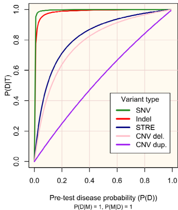
302 303 Figure 2. Probability of disease D following a positive genetic test result for marker M ( P(D|T) ) according to pre-test disease 304 probability ( P(D) )
