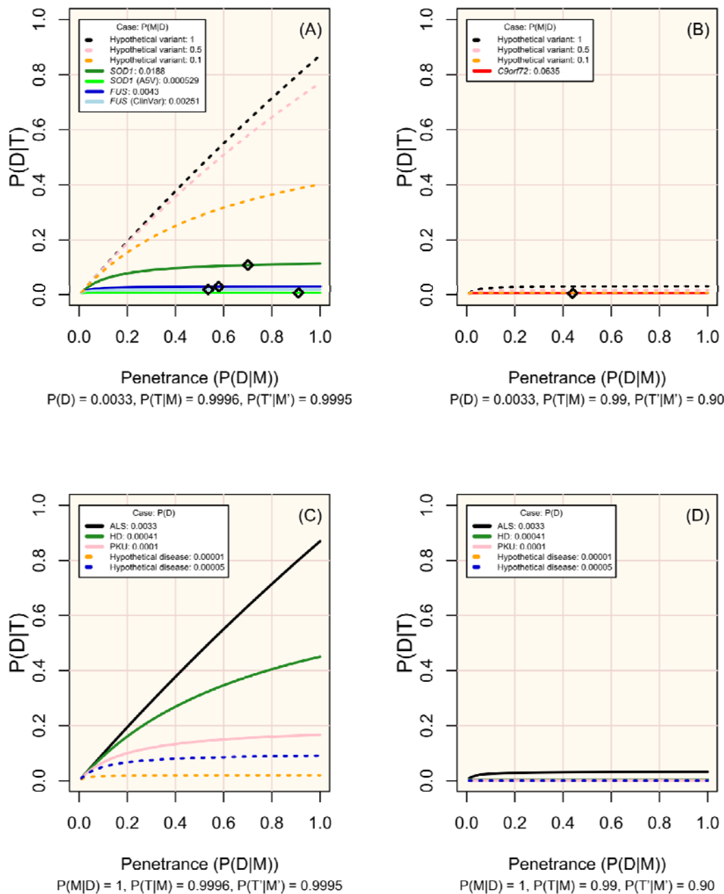
Figure 3. Change in disease risk following a positive test result for a marker of increased disease risk ( P(D|T) ) according to penetrance ( P(D|M) )
