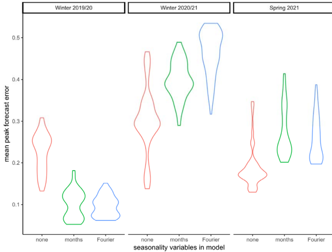
Figure 1: Violin plot of mean peak error by validation season, stratified by seasonality variant.
