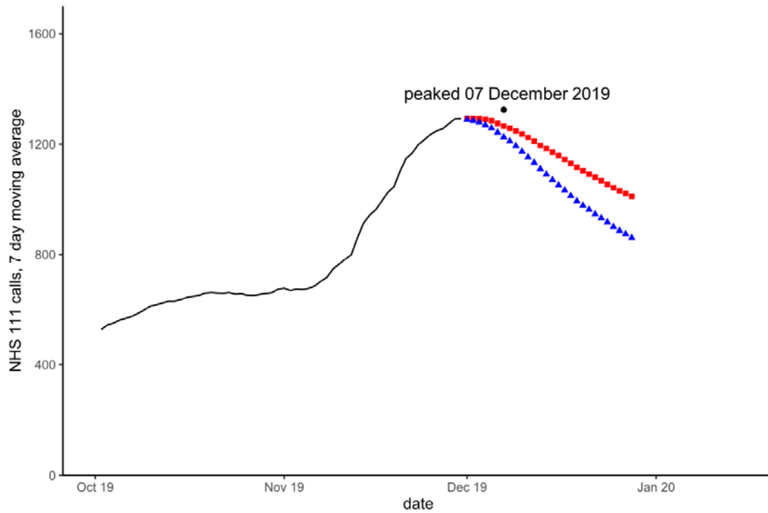
Figure 2: Forecasts for NHS 111 cough calls in under 5 years on 30 November 2019. Blue triangles are forecast with modelled seasonality, red squares without seasonality. The black dot and date refer to the actual observed peak of activity during the period.
