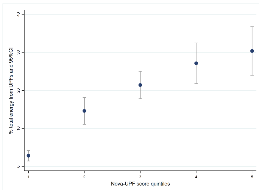
Figure 5: Mean dietary share of UPF obtained from full 24-h recall according to Nova-UPF score intervals
