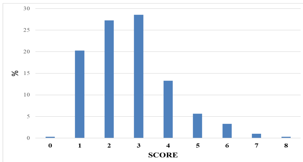
Figure 4: Nova-UPF score distribution.
