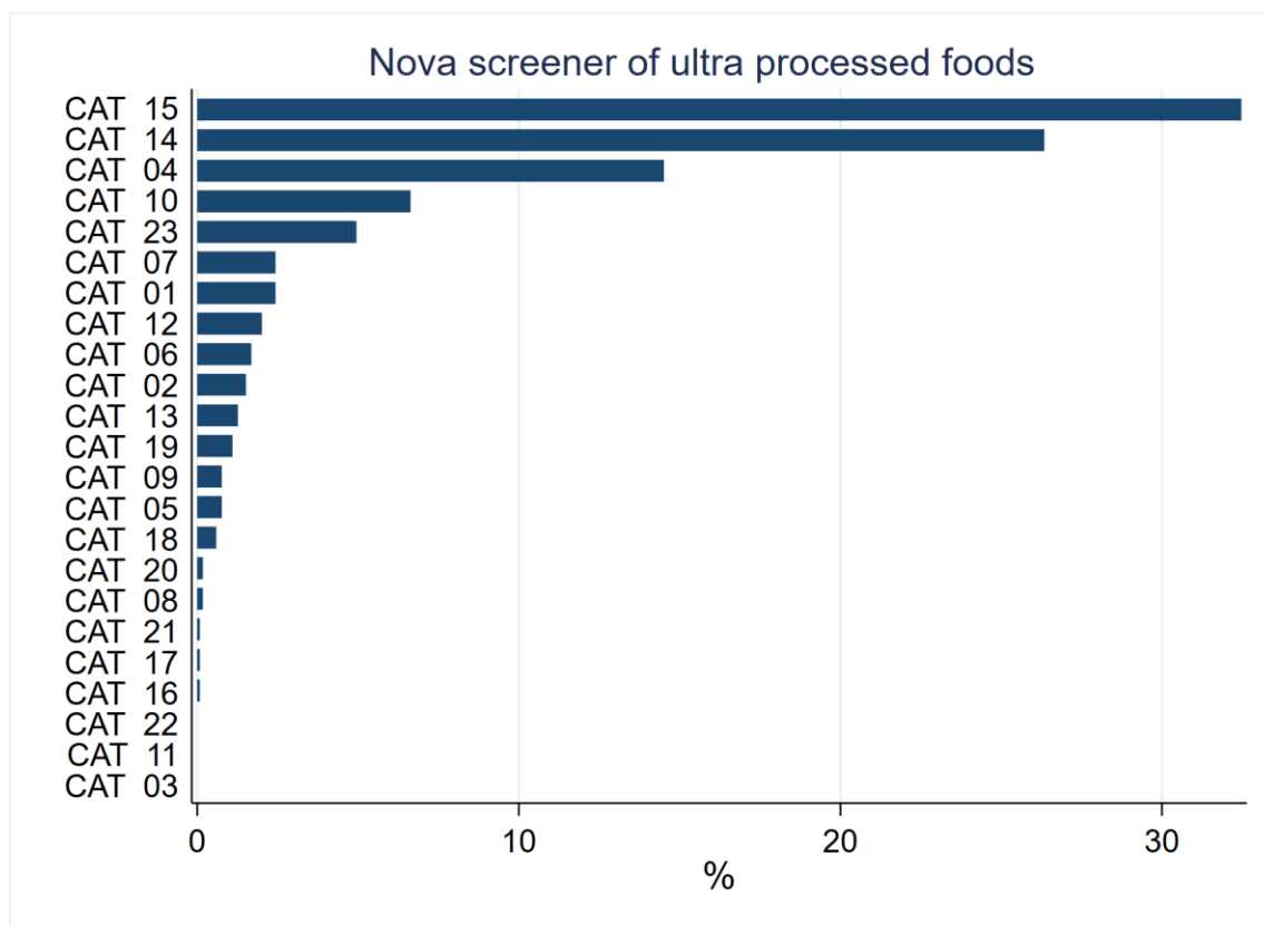
Figure 3: Consumption frequencies of ultra-processed food subcategories.
