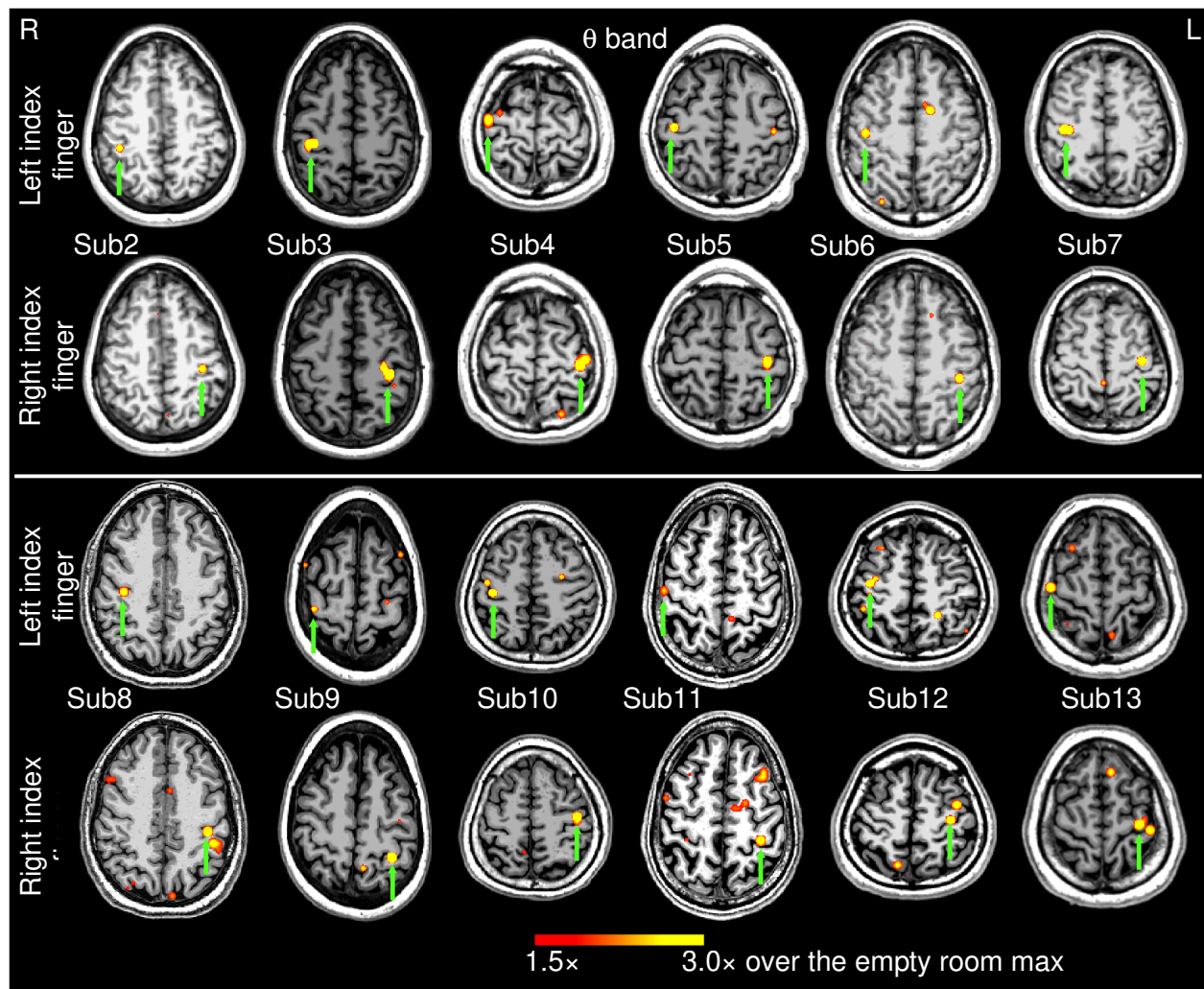
Figure 3: Movement-related theta-band EMG-projected MEG source images for the remaining 12 healthy subjects. Significant primary motor cortex sources (green arrows) contralateral to the left or right self-paced (~1 min) index finger movements. The color bar shows the activity threshold at \geq 1.5\times of the empty room maximum value, and a saturation level at 3.0\times . Sub = subject
