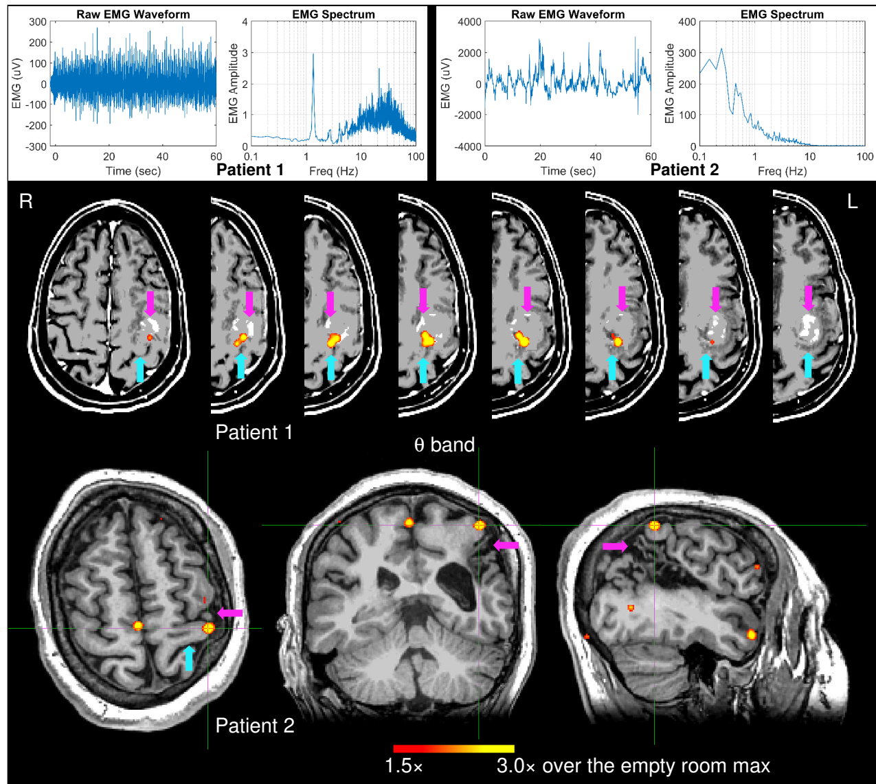
Figure 5: Top panel: EMG waveform and spectrum from two patients with brain lesions when they performed right self-paced (~1 min) index-finger movements. Bottom panel: Movement-related theta-band EMG-projected MEG source images for the two patients. Primary motor cortex sources contralateral to right self-paced index-finger movements were significant in both patients. In Patient 2, the M1 was also indicated by the crosshairs. The magenta arrows indicate the brain lesions, and the cyan arrows indicate the central sulcus.
