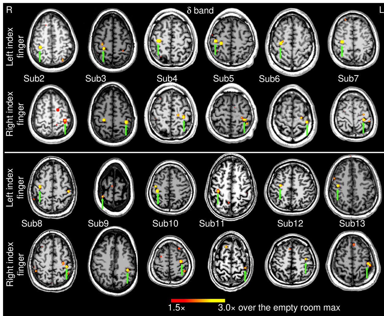
Figure 2: Movement-related delta-band EMG-projected MEG source images for the remaining 12 healthy subjects. Significant primary motor cortex sources (green arrows) contralateral to the left or right self-paced (~1 min) index finger movements. The color bar shows the activity threshold at \geq 1.5\times of the empty room maximum value, and a saturation level at 3.0\times . Sub = subject
