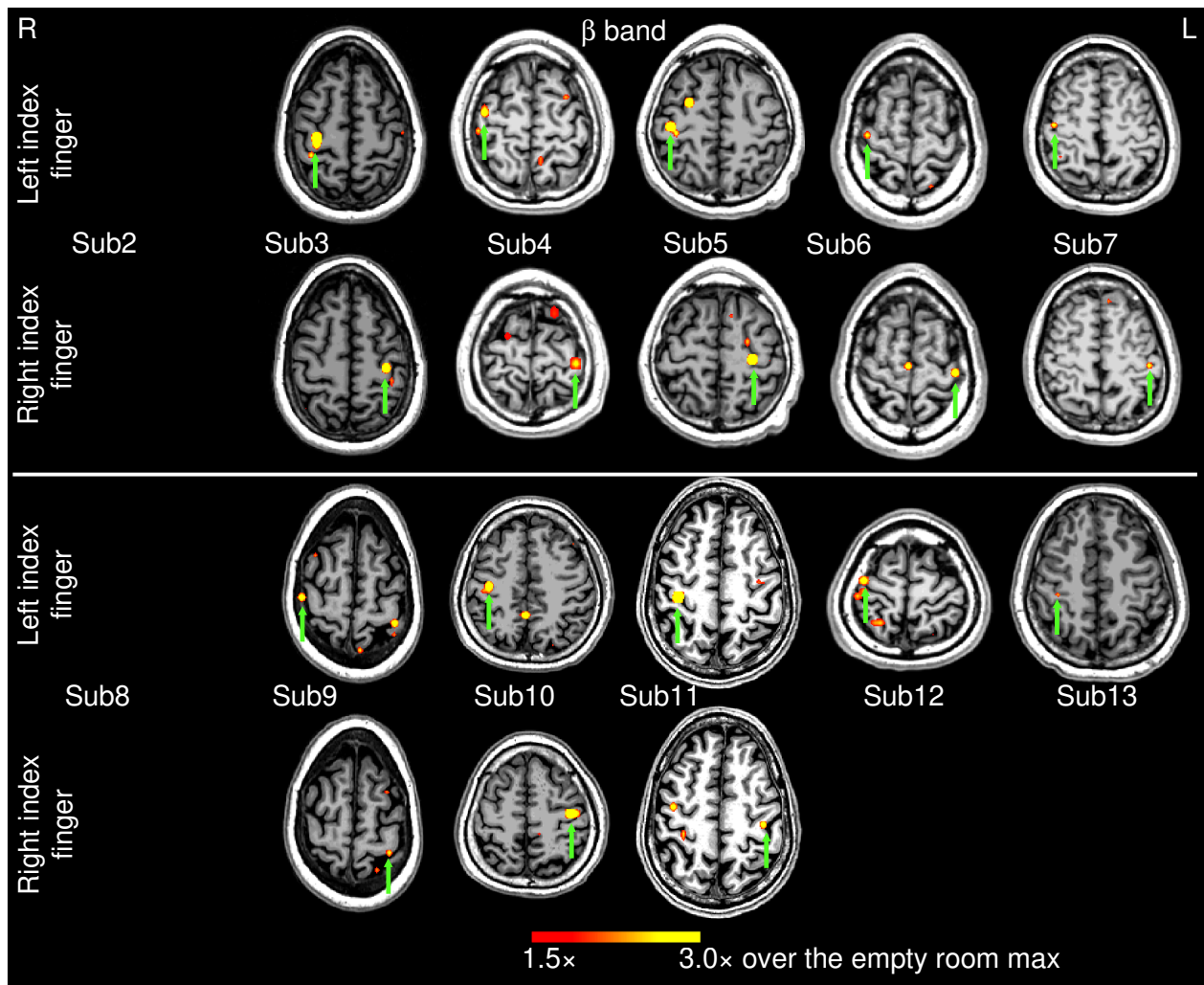
Figure 4: Movement-related beta-band EMG-projected MEG source images for the remaining 12 healthy subjects. Primary motor cortex sources (green arrows) contralateral to self-paced (~1 min) left or right index finger movements were significant in 18 out of 24 cases. The color bar shows the activity threshold at \geq 1.5\times of the empty room maximum value, and a saturation level at 3.0\times . In 6 cases, contralateral primary motor source activity did not reach threshold. Sub = subject
