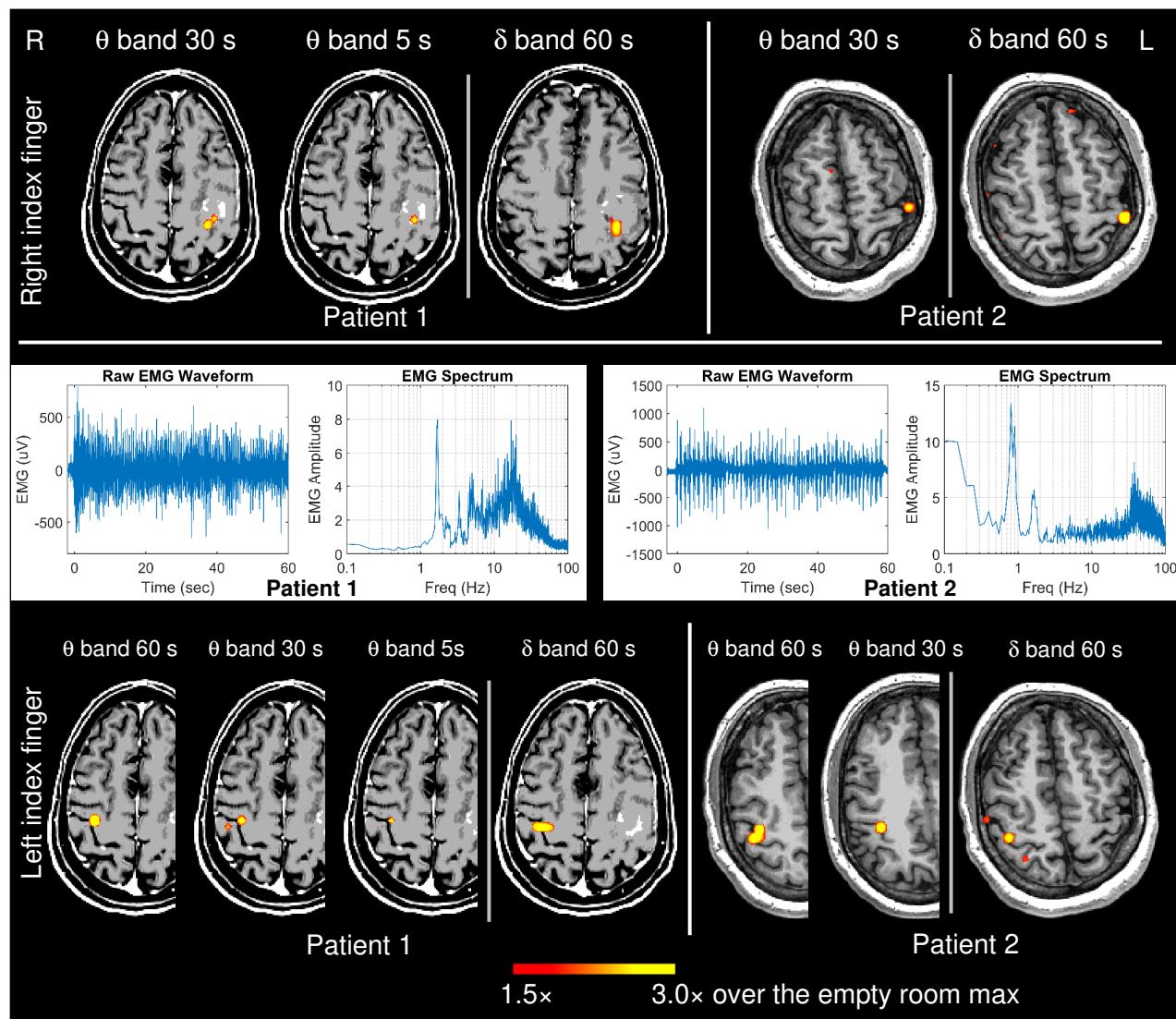
Figure S2: This figure provides supplementary results to Figure 5 in the main text. Top Panel: EMG-projected MEG source images of M1 cortex in the affected left hemispheres due to right finger movement (affected hand) from the two clinical patients in theta and delta bands. In the theta band, M1 was localized in 30 sec and 5 sec time windows in Patient 1, but only the 30 sec time window in Patient 2. Delta-band M1 cortical activity (1 min EEG recordings) in the damaged hemisphere was localized in both patients. Middle Panel: the EMG waveforms and spectra from the left index finger movement (unaffected hand). Bottom Panel: EMG-projected MEG source images of M1 in the unaffected right hemispheres due to left finger movement from the patients in theta and delta bands. In Patient 1, theta-band M1 cortex activity was localized in the 60 sec, 30 sec and 5 sec time windows. In Patient 2, theta-band M1 activity was localized only in the 60 sec and 30 sec time windows. Delta-band M1 activity (1 min EEG recordings) was localized in the unaffected hemisphere in both patients.
