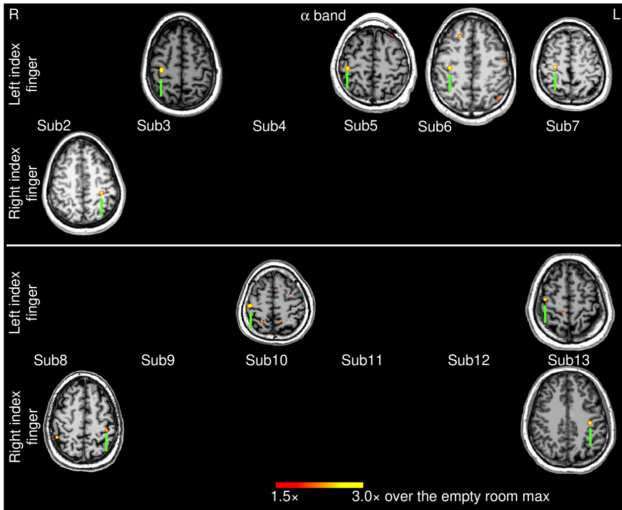
Figure S1: Movement-related alpha-band EMG-projected MEG source images for the remaining 12 healthy subjects. Significant primary motor cortex sources (green arrows) contralateral to left or right self-paced (~1 min) index finger movements. The color bar shows the activity threshold at 1.5 \times of the empty room maximum value, and saturation level at 3.0 \times . In 6 cases, contralateral primary motor source activity at or above the threshold was not observed. Sub = subject
