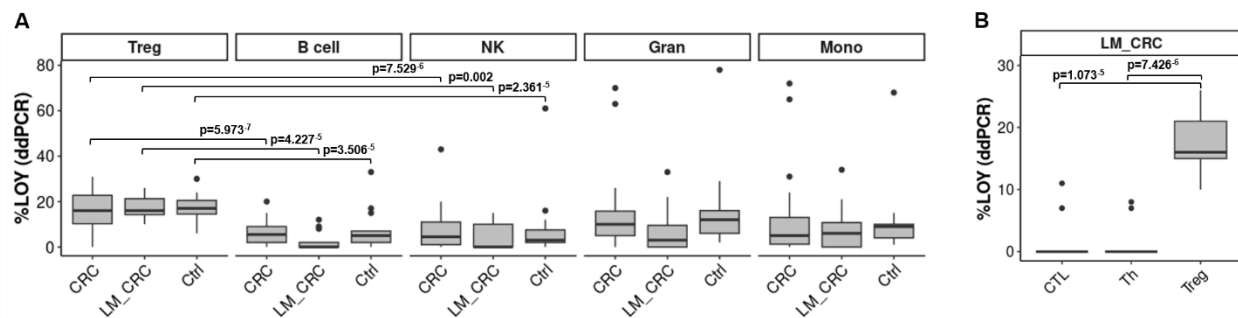
Fig. 4. Experimental detection of the distribution of LOY in sorted blood cells from patients with primary CRC, liver metastases of CRC and controls.
