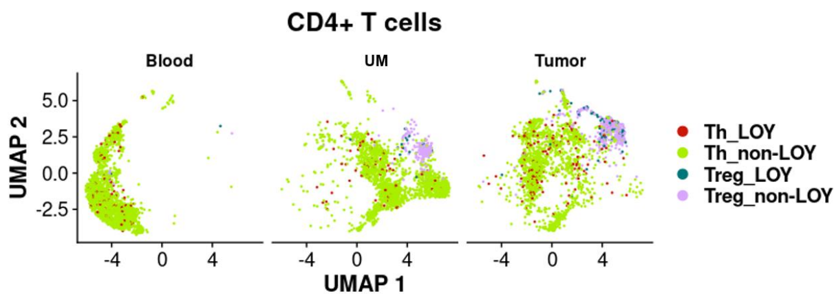
Fig. 3. Computational analysis of distribution of LOY CD4+ T lymphocytes in different tissues of CRC patients. CD4+ T cells were extracted from the tumor, uninvolved margin (UM) and blood samples obtained from four CRC patients (Zhang et al., 2020) and categorized into Th and Tregs. Next, LOY-cells were defined based on the lack of expression of MSY-specific genes.
