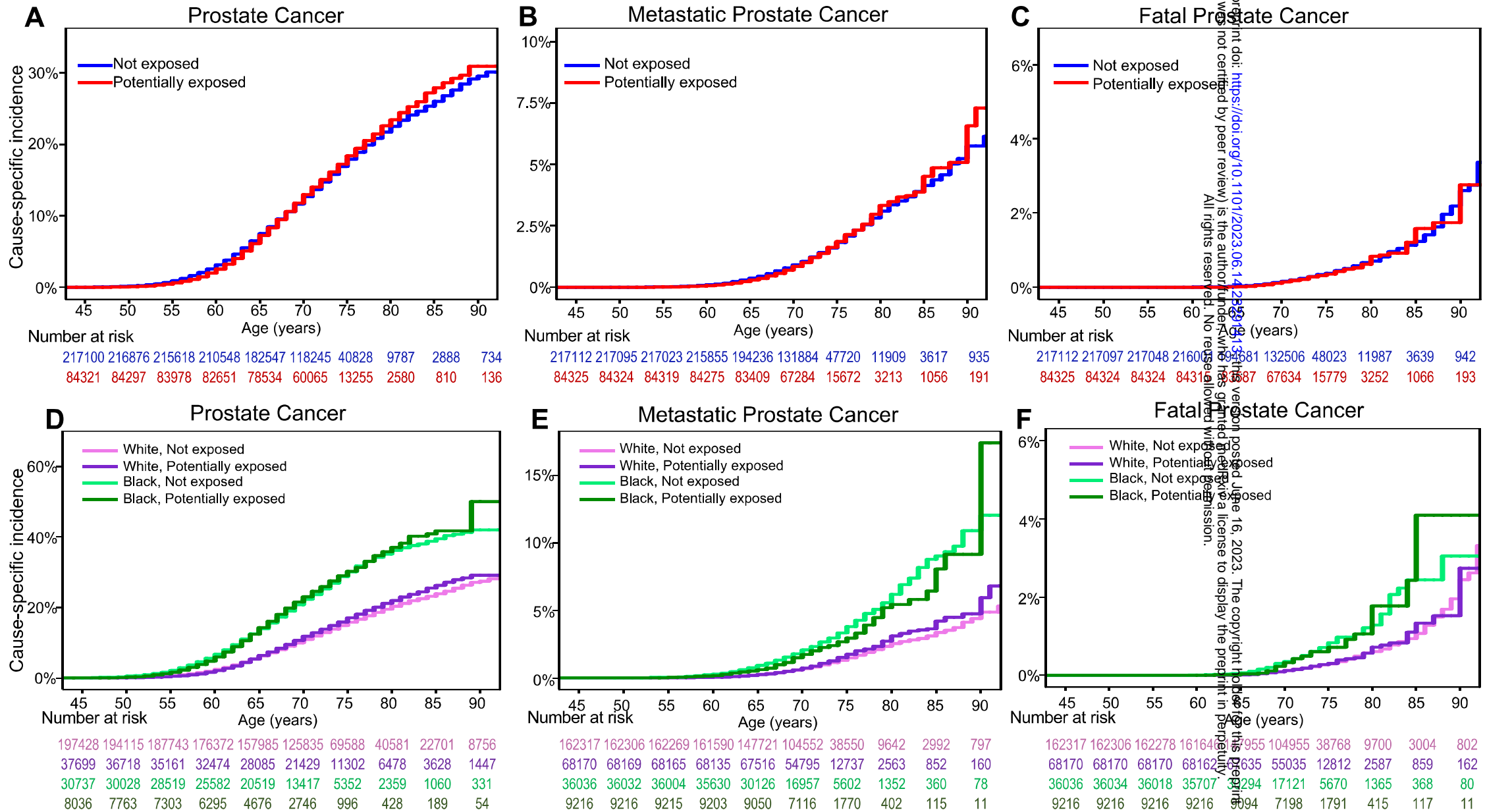
Figure 1. Million Veteran Program (MVP) Cause-specific Cumulative Incidence based on Agent Orange exposure. Cause-specific cumulative incidence among MVP participants on active duty during the Vietnam War, stratified by Agent Orange exposure status (top row) and stratified by self-reported race (bottom row) for (A, D) all prostate cancer, (B, E) metastatic prostate cancer, and (C, F) fatal prostate cancer. “White” indicates Non-Hispanic White participants, and “Black” indicates Black and Hispanic Black participants.
