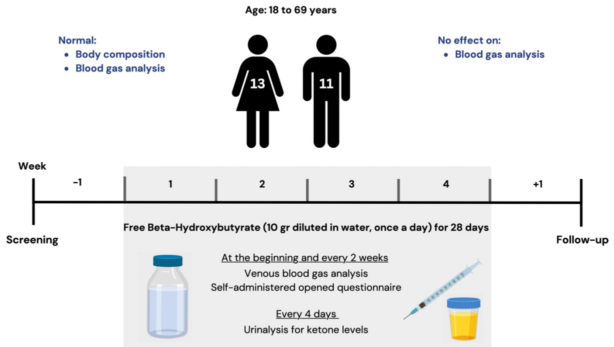
Figure 1. Study Workflow.
