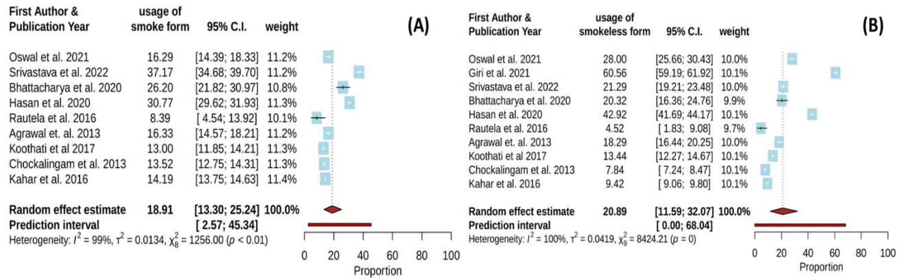
Figure 4: Forest Plot- overall current usage of (A) Smoke form, (B) smokeless form among general Indian population in the period of 2010 – 2022
