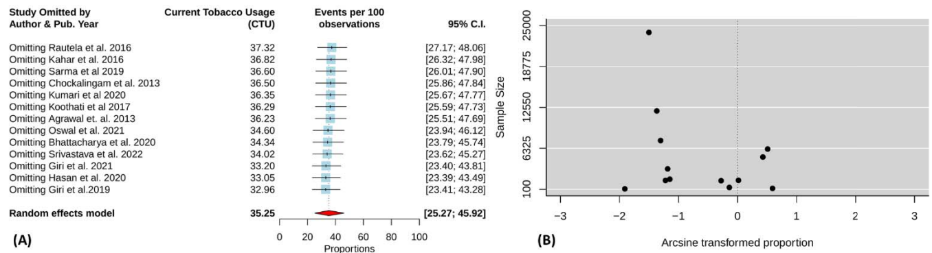
Figure 5: (A) Leave-one-out analysis establishing sensitivity of overall CTU estimate; (B) Assessment of publication bias- funnel plot
