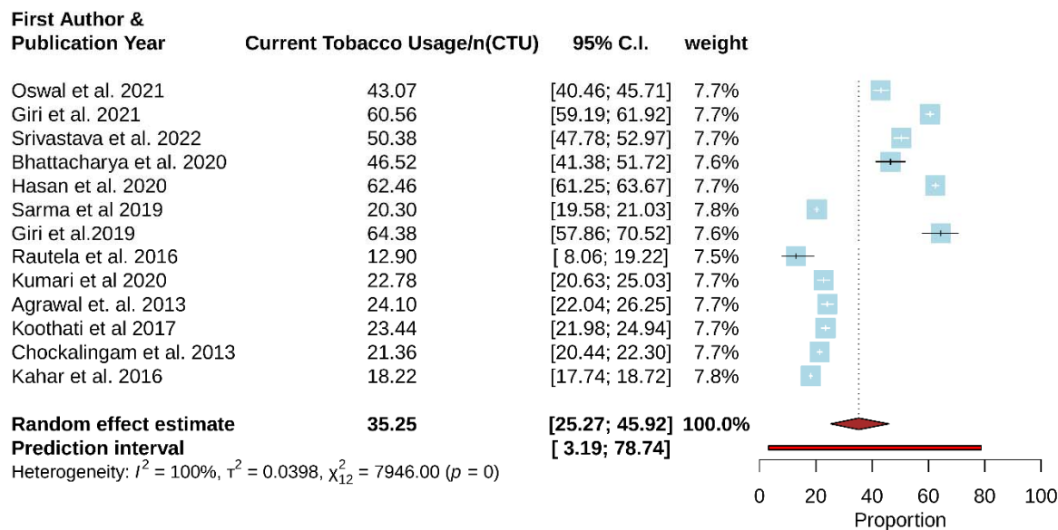
Figure 3: Forest Plot- overall current tobacco usage among general Indian population between period 2010 – 2022
