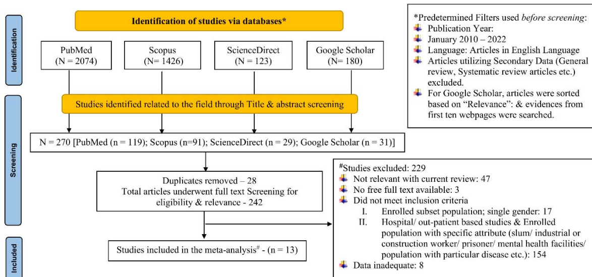
Figure 1: PRISMA flowchart for selection and inclusion of studies in the review
