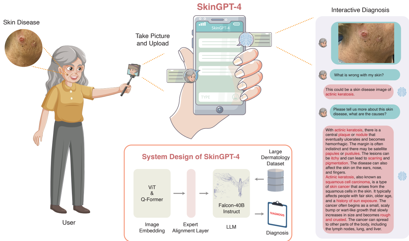
Fig. 1. Illustration of SkinGPT-4. SkinGPT-4 is the world's first interactive dermatology diagnostic system based on multimodal large language models. To implement SkinGPT-4, we have designed a new framework that aligned a pre-trained vision transformer with a large language model named Falcon-40B-Instruct. SkinGPT-4 was trained on a vast collection (52,929) of both public and in-house skin disease images, accompanied by clinical concepts and doctors' notes. With SkinGPT-4, users could upload their own skin photos for diagnosis, and SkinGPT-4 could autonomously determine the characteristics and categories of skin conditions, perform analysis, provide treatment recommendations, and allow interactive diagnosis. On the right is an example of interactive diagnosis.
