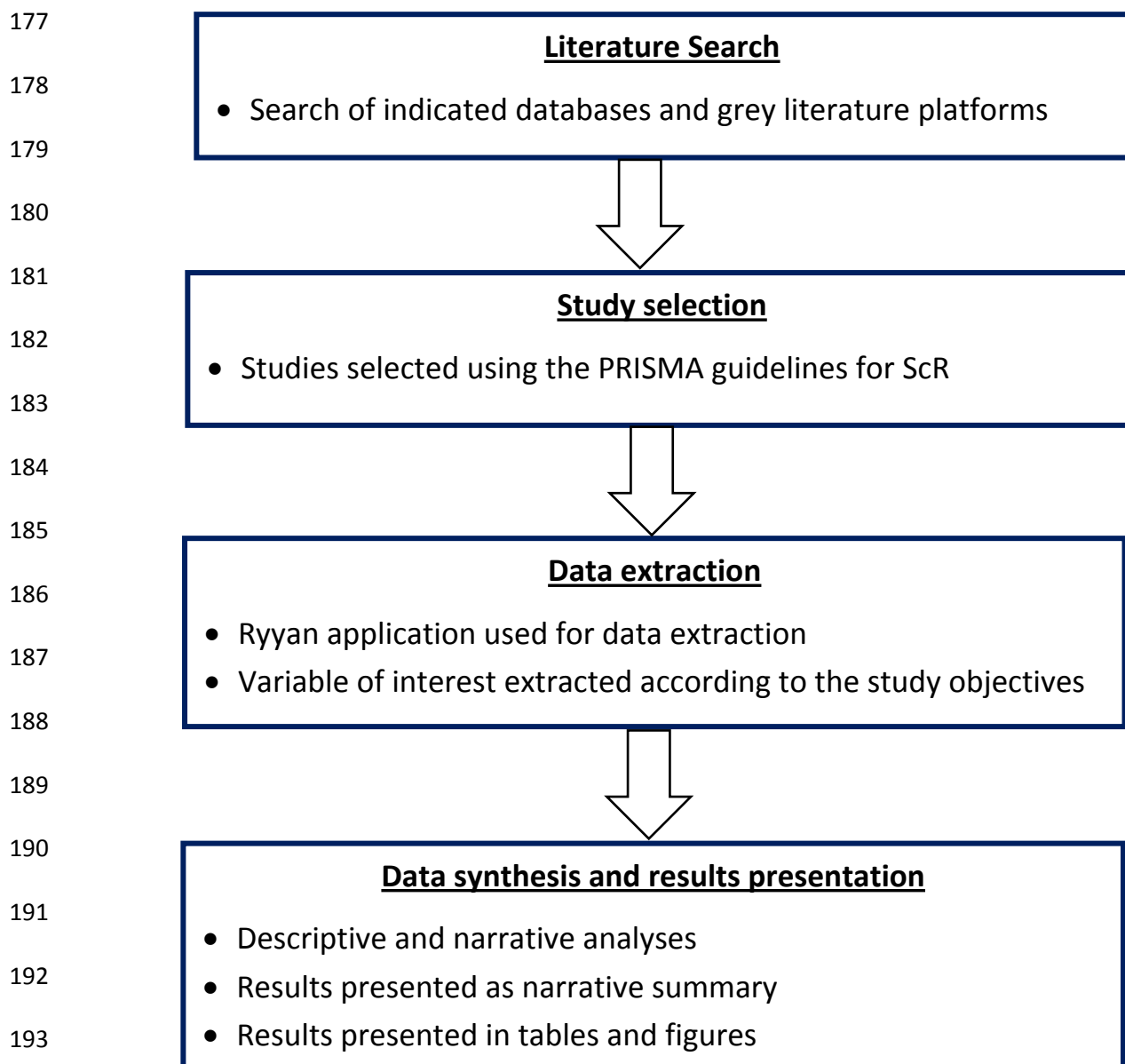
175 Figure 1: Flow diagram for the scoping review methodology on gender differences in 176 antibiotics use behaviour and access to antibiotics in LMICs
