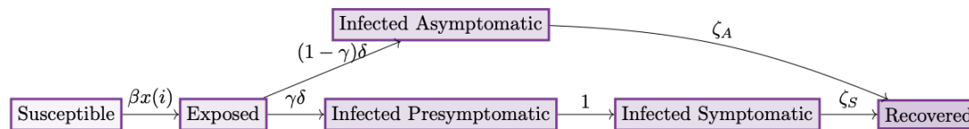
Figure 3: Extended SEIR model used in the paper. Arrows indicate the movement between the states with the rate of this movement written on the arrow.
