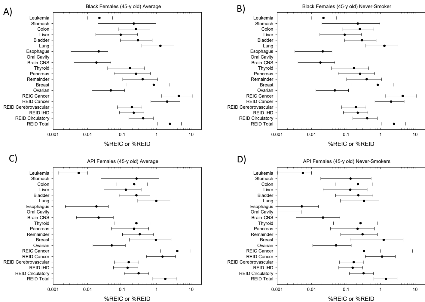
Figure 5. Tissue specific risks and 95% confidence intervals for Females on 80-day lunar missions. A) Black average population, B) Black never-smokers, C) Asian-Pacific Islander (API) average populations, and D) API never-smokers.
