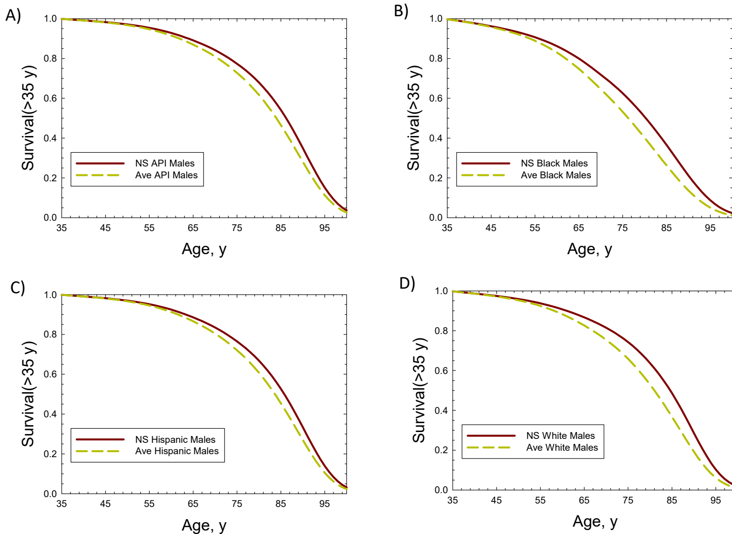
Figure 3. Conditional survival probabilities for Males with entry at age 35-y versus age comparing US average and Never-Smokers (NS) for A) Asian-Pacific Islanders, B) Black, C) Hispanic and D) Whites.
