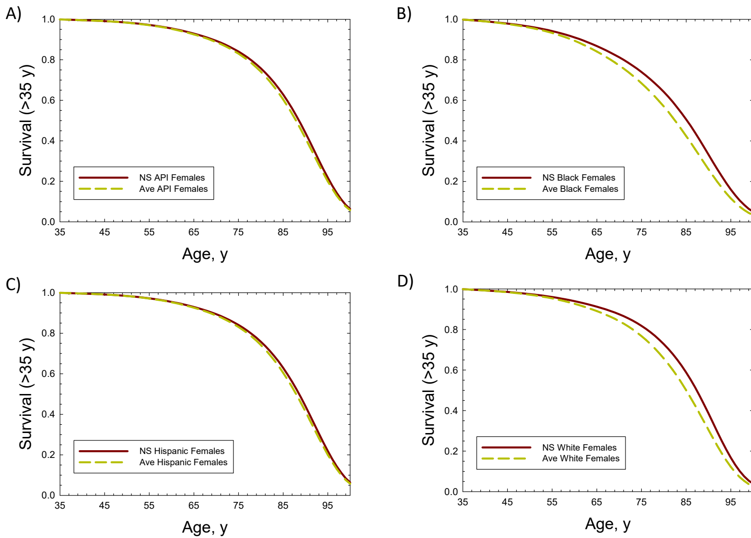
Figure 1. Conditional survival probabilities for Females with entry at age 35-y versus age comparing US average and Never-Smokers (NS) for A) Asian-Pacific Islanders, B) Black, C) Hispanic and D) Whites.
