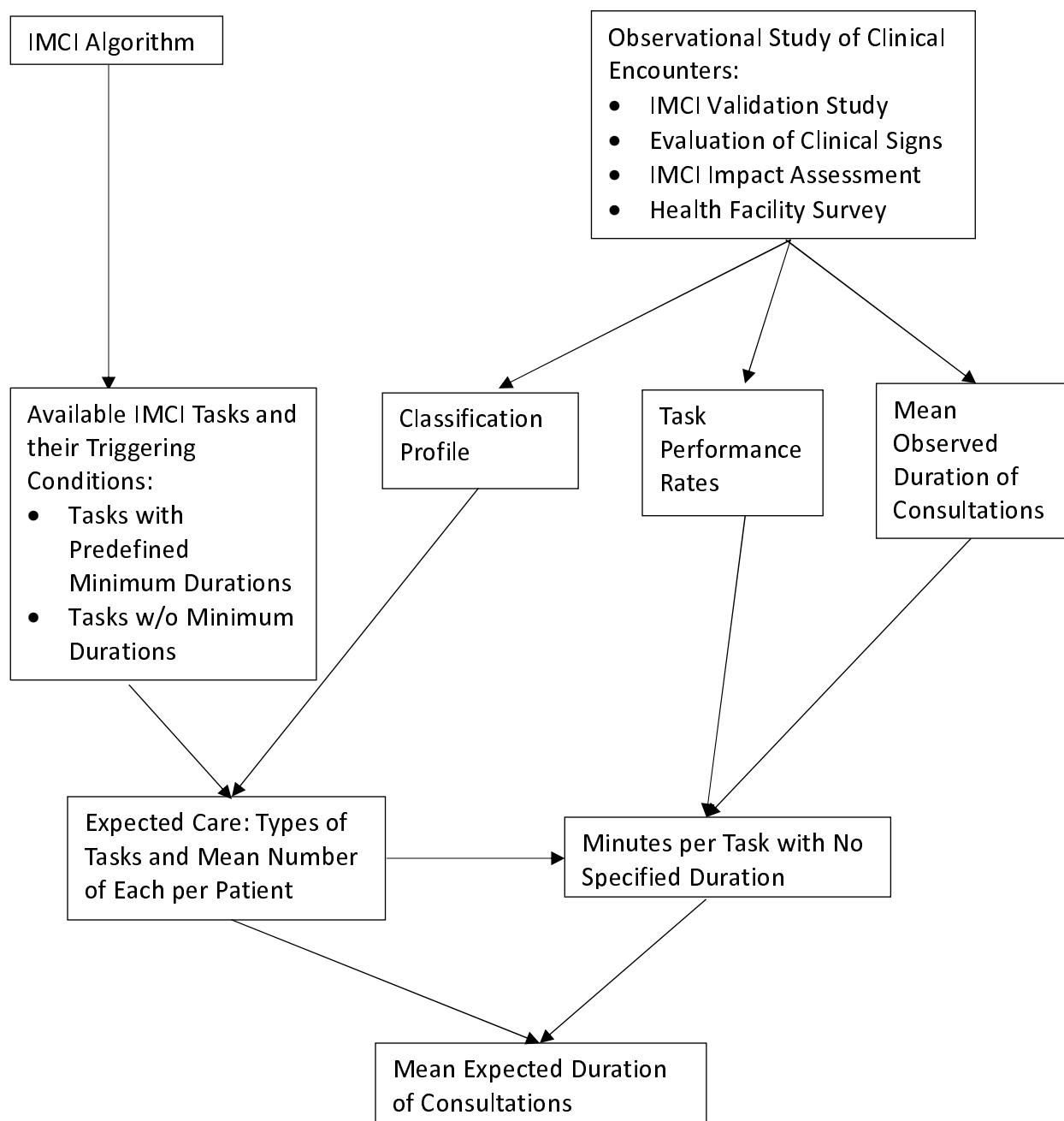
Figure 1: Analytical Framework
