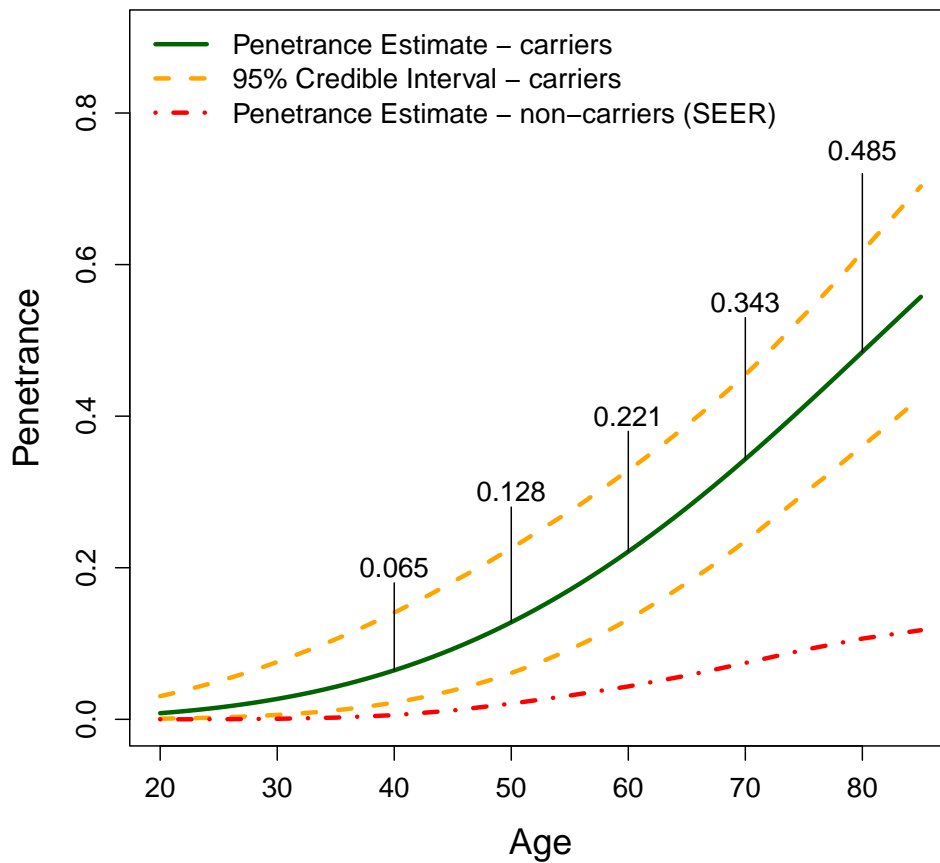
Figure 1: Penetrance estimate of BC for PALB2 mutations.
