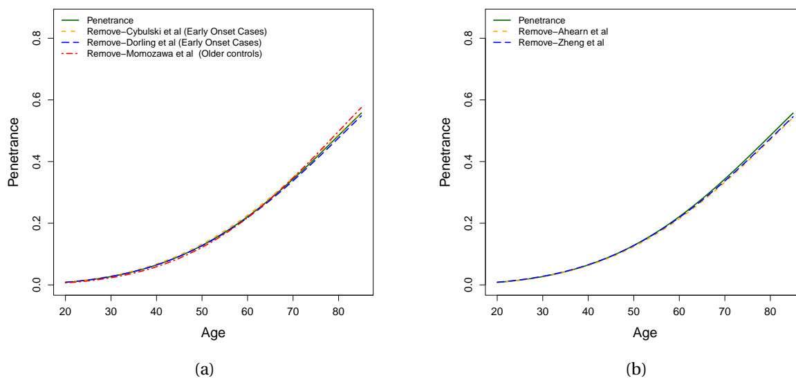
Figure 3: Results of sensitivity analysis: (a) Removing studies with early onset cases or controls restricted to older ages, one at a time. (b) Removing Ahearn et al. (2022) and Zheng et al. (2018) one at a time.
