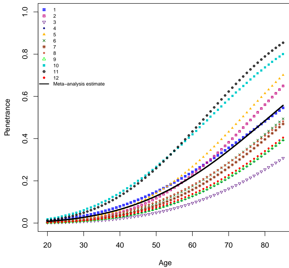
Figure 2: Approximate penetrance curves (Weibull distributions) for each of the 12 studies: The number in the legend corresponds to the study index in Table 1.
