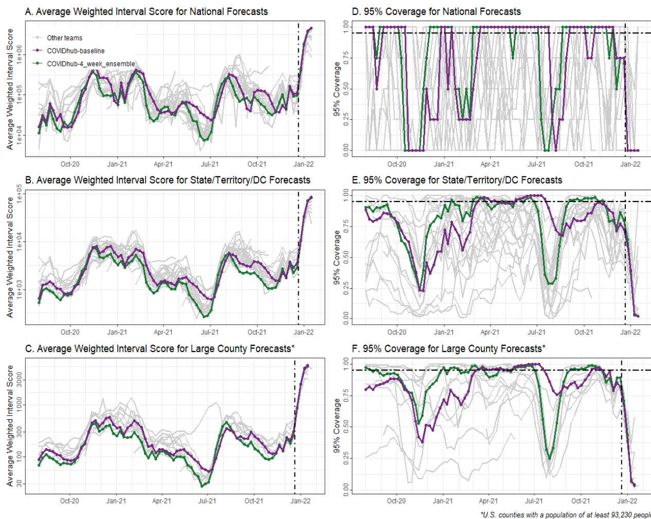
Figure 6: Forecast accuracy over time, aggregated by geographic units, forecast horizon, and prediction date. Panels A-C show average Weighted Interval Score (WIS); panels D-F show 95% prediction interval coverage. The black, dashed vertical line in all panels shows the date that public communication of the case forecasts was paused. The black, dashed horizontal line in panels D-F shows nominal 95% interval coverage. National level forecasts are presented in A and D, state/territory/DC forecasts in B and E and large county level forecasts in C and F.
