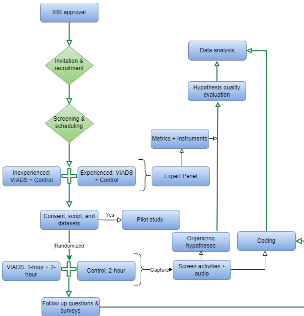
Figure 1 Study flow for the data-driven hypothesis generation
