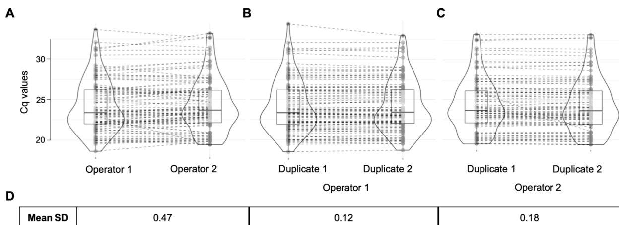
272 Figure 2 – RNA extraction validation using RPL13A gene expression. The RNA extraction method was 273 validated by two different operators ( p = 0.27 , Paired Student's t-test) ( A ). Moreover, each operator 274 performed the assays in duplicate: operator 1 ( p = 0.99 , Paired Student's t-test) ( B ) and operator 2 275 ( p = 0.13 , Paired Student's t-test) ( C ). The mean SD between operators and within operators is also
