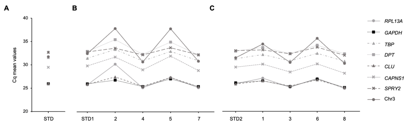
401 Figure 5 – Robustness of the RT-qPCR reactions included in the HepatoPredict kit. Representation of Cq 402 mean values for each condition ( Table 1 ) of each target included in the HepatoPredict kit. The original 403 condition (STD) ( A ) was compared with all other conditions (1 to 8) and no statistically significant 404 differences were observed (Dunn's multiple comparisons test). Moreover, conditions with the same 405 annealing temperature were compared with the respective STD condition: ( B ) STD1 was compared with 406 condition 2, 4, 5 and 7 while ( C ) STD2 was compared with conditions 1, 3, 6, and 8. No statistically 407 significant differences were observed (Dunn's multiple comparisons test).
