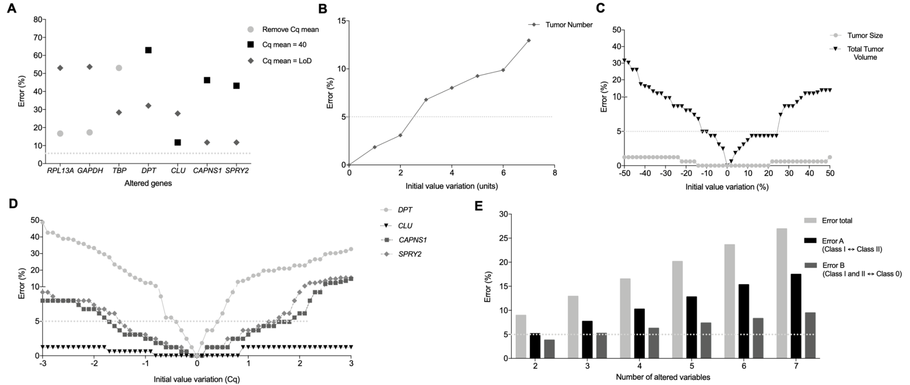
469 Figure 6 – Robustness of the HepatoPredict algorithm. Representation of errors associated with the univariate alteration of Cq mean values from each molecular 470 variables before normalization (A), with the univariate alteration of the tumor number (B), or tumor size or total tumor volume (C). Errors associated with the 471 univariate alteration of the molecular variables after normalization (D). Multivariate analyses of the HepatoPredict algorithm for distinct combinations of 472 variables, ranging from 2 to 7 variables (E). The dashed line in light grey represents the errors at 5%.
