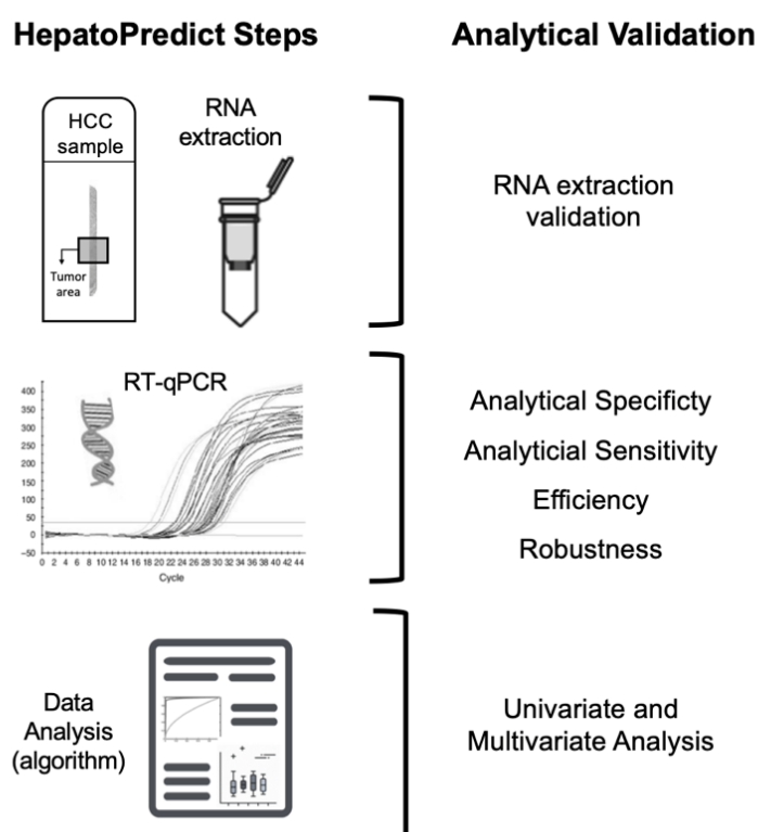
83 Figure 1 – HepatoPredict kit Analytical Validation. The HepatoPredict kit intends to predict tumor 84 recurrence after a liver transplant in patients with HCC. The HepatoPredict kit uses FFPE HCC samples 85 from which the RNA is extracted and subsequently used as a template in 1-step RT-qPCR reactions
