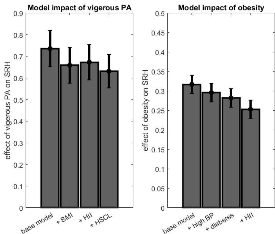
Figure 3: Effect on model parameters of adjusting for confounders and other covariates. Note that the bars show the adjusted impact of PA (left panel) and BMI (right panel), respectively, on SRH across models that adjust for increasingly more variables. The effect of PA is summarised with the difference between those who exercise intensely \geq 4 times per week and those who exercise < 1 time per week with mild intensity. The effect of BMI is summarised with the difference between the obese and the normal category. The effects are shown together with 95% confidence intervals. The models are nested and increasing in size going left to right. Both baseline models control for sex, age, current smoking, and education level. The BMI baseline model also controls for PA.
