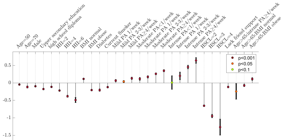
Figure 1: Effects on Self-Rated Health (SRH) in the fully adjusted mixed effects model. SRH is modelled as a continuous variable, with one unit increase representing a one-level change on the 4-level SHR scale, such as from “very bad” to “bad” or “good” to “very good”. Interaction effects are denoted with “:” (the three parameters furthest to the right). Reference categories are mild PA; PA <1 time per week; overweight; college/university level education. HII, HSCL, and age are modelled as continuous variables. Their effects are sampled at various points with baseline values being 0 (HII), 0 (HSCL), and 30 years of age, respectively. The recommended cut-off for significant mental health symptoms is HSCL=1.85. Examples of combinations of comorbidities that correspond to HII-levels 2, 4, and 6, respectively, are 1. Heart attack, 2. Heart attack and Cerebrovascular stroke, and 3. Heart attack, Cerebrovascular stroke, and Asthma.
