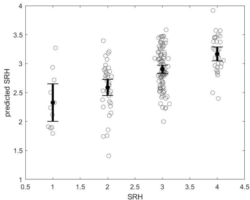
Figure 4: Test-set predictions of SRH vs actual SRH values for 200 Tromsø 7 participants. Only participants who participated in Tromsø7, but not Tromsø6, were included in the test set to ensure independence. Random values have been added to the x-coordinates for visual clarity. The intervals are 95% confidence intervals for the mean of each set of predictions.
