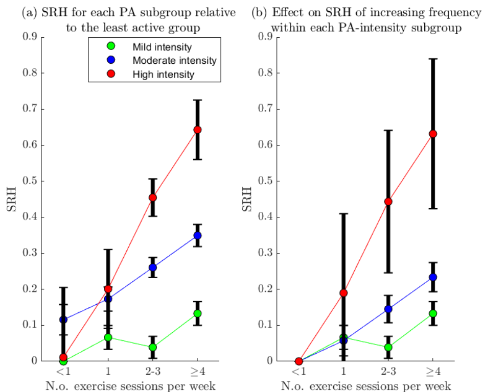
Figure 2: Joint effect of Physical Activity Frequency and Intensity on SRH in the adjusted model. The figures show average SRH (in the fully adjusted model) for different PA subgroups relative to different reference groups. In panel (a), all effects are presented with the least physically active group (mild intensity <1 per week) as the reference group. In Panel (b), the effect on SRH of exercising with intensity i and frequency f is represented relative to those that exercise with with intensity i < 1 per week, so tracing each interpolating line shows the effect of increasing exercise frequency from the lowest frequency (<1 per week) to the frequency specified on the x-axis whilst holding the exercise intensity fixed at the level specified by the colour.
