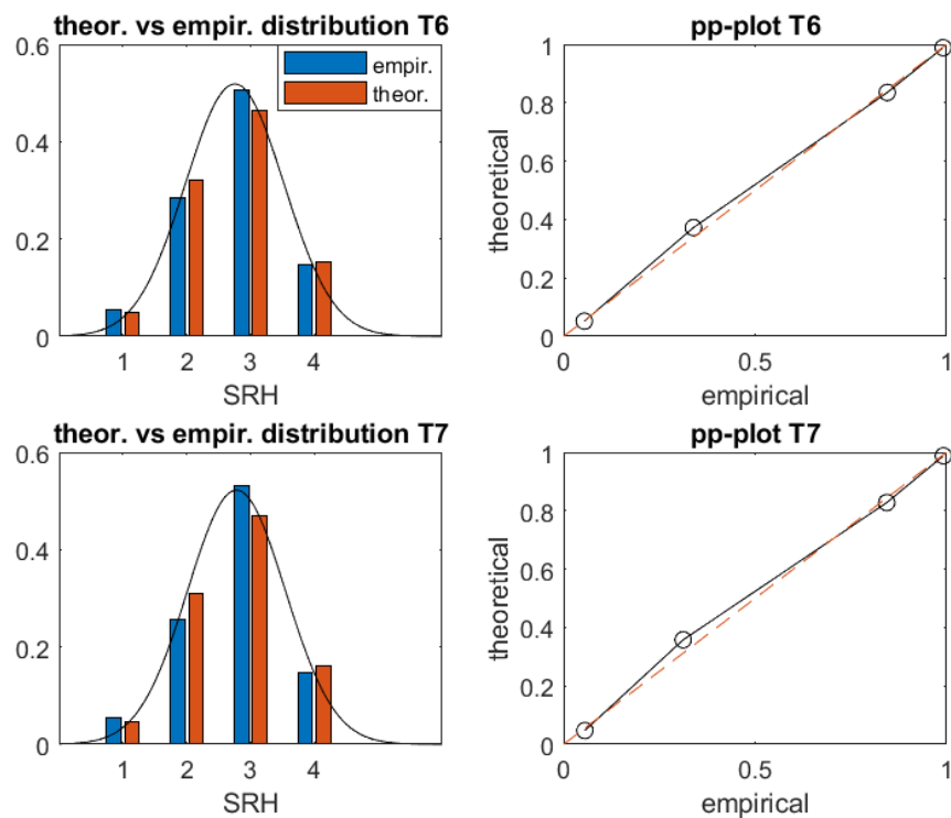
Figure 5: Theoretical vs fitted normal distribution of SRH in Tromsø 6 and Tromsø 7. The theoretical probabilities for each of the 4 SRH levels were defined as the probability mass over the four bins defined by the bin-boundaries 1.5, 2.5, and 3.5. The right-hand figures are probability-probability plots showing the empirically vs theoretically estimated probabilities of SRH \leq i for i=1, 2, 3 and 4.
