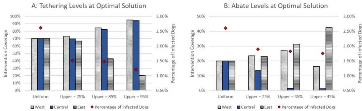
Figure 4 (A) Tethering levels in all clusters under different intervention upper bounds with Abate fixed at 50%; (B) Abate levels in all clusters under different upper bounds with tethering fixed at 95%.
