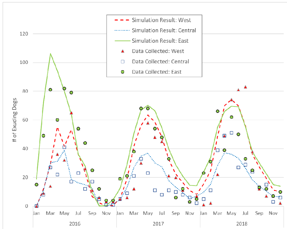
Figure 3 Observed number of dogs infected by cluster for years 2016-2018 and simulated dogs infected from the MWS model.
