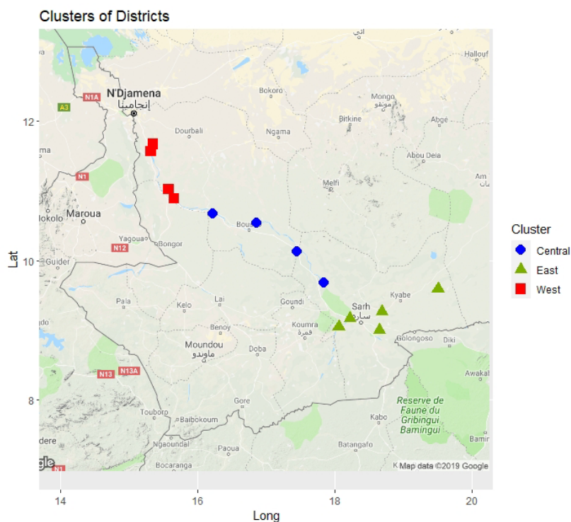
Figure 1 Districts in Chad by computed clusters.
