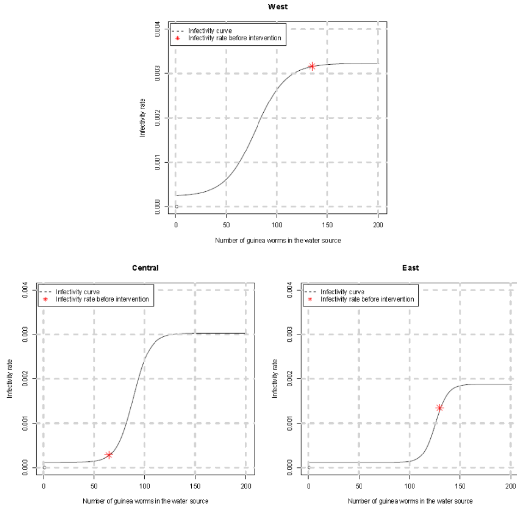
Figure 2 Infectivity curves for the West, Central, and East clusters.
