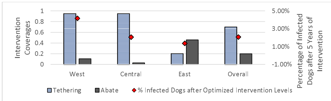
Figure 5 Optimized strategy with average resource levels of 70% and 20% for tethering and Abate, respectively.
