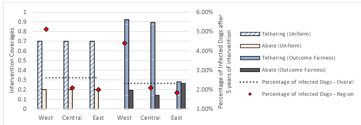
Figure 6 Optimized strategies by cluster under the uniform strategy and with constraints to maximize outcome fairness.
