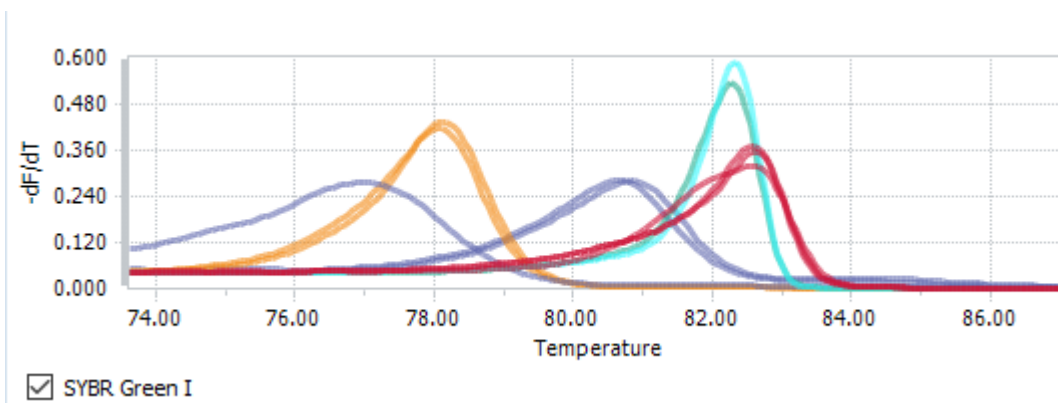
184 Figure 3. High resolution melting peaks for EV and CCHFV (red), RVFV (turquoise), MV 185 (yellow) Short LV and \beta -globin (81°C purple), Long LV (77°C purple). Colours are grouped 186 by melting temperature (°C).
