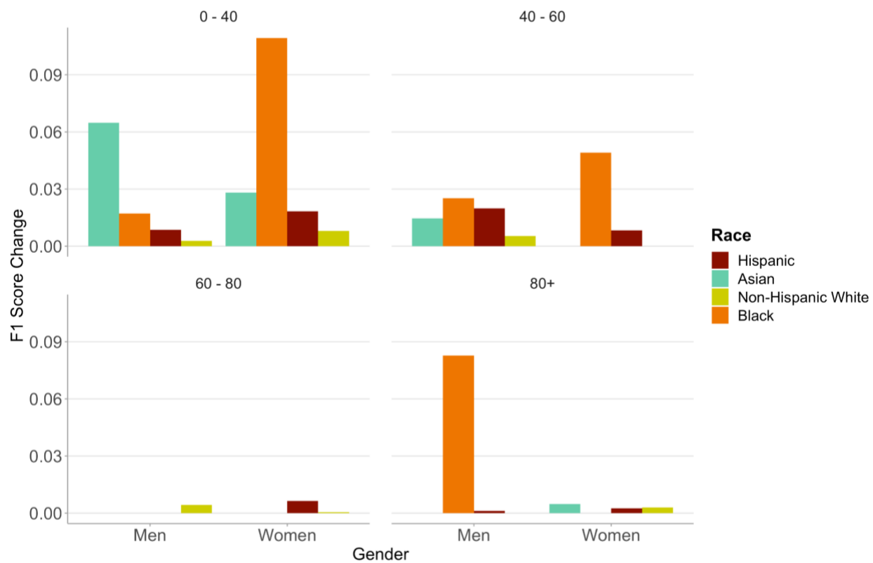
Figure 6. Changes in F1-Score when using probability thresholds individualized for race, age, and gender subgroups
