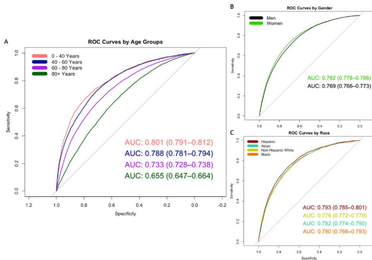
Figure 1. Receiver operator characteristic (ROC) curves and area under the curve (AUC) stratified by race, age, and gender
