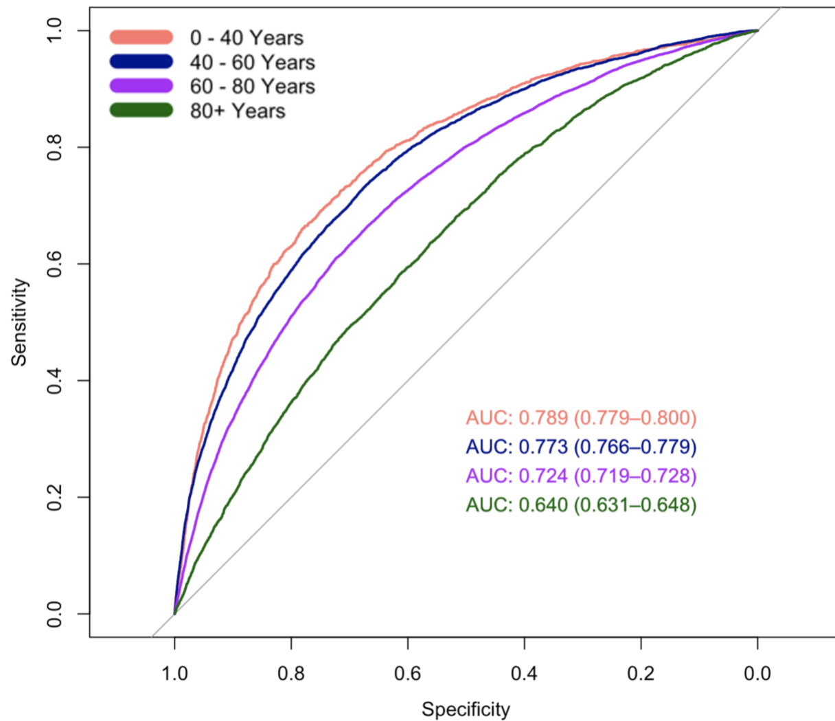
Supplementary Figure 6. ROC curves from models trained and tested separately by age group
