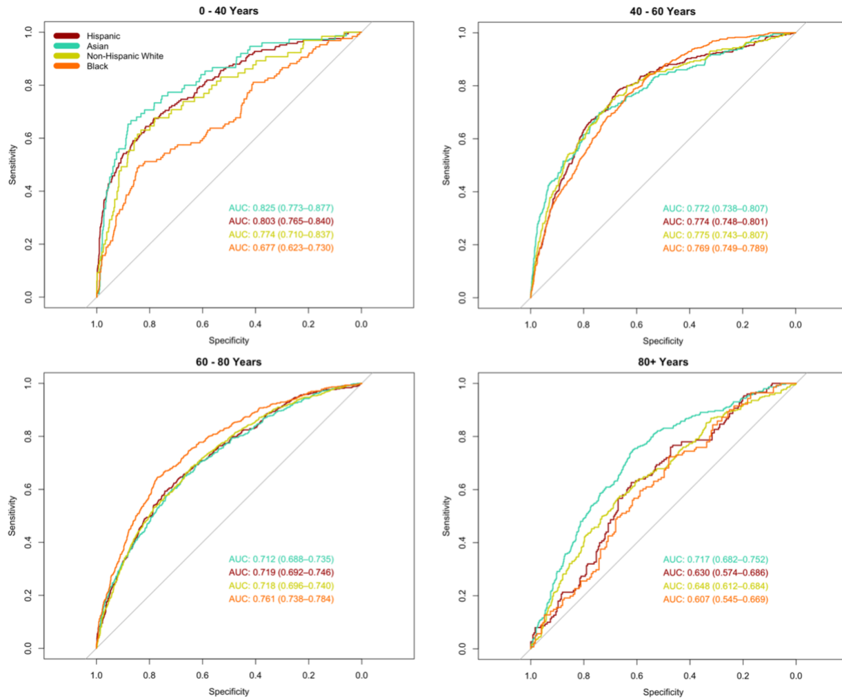
Supplementary Figure 4. ROC curves stratified by race and age from a model trained on a dataset with equal racial representation.
