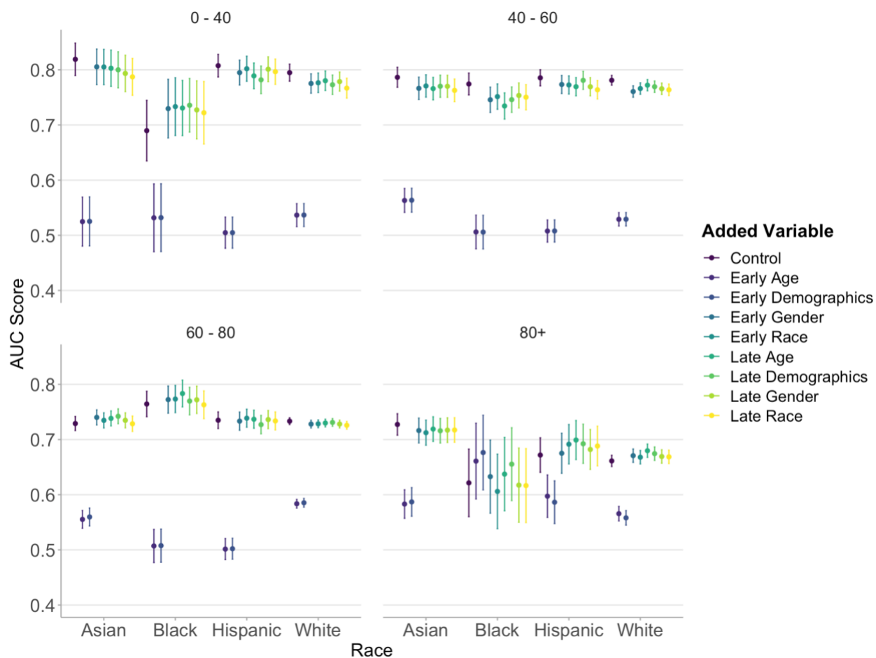
Figure 5. AUC values by race and age groups with integration of age, race, and gender variables at earlier and later points in model architecture
