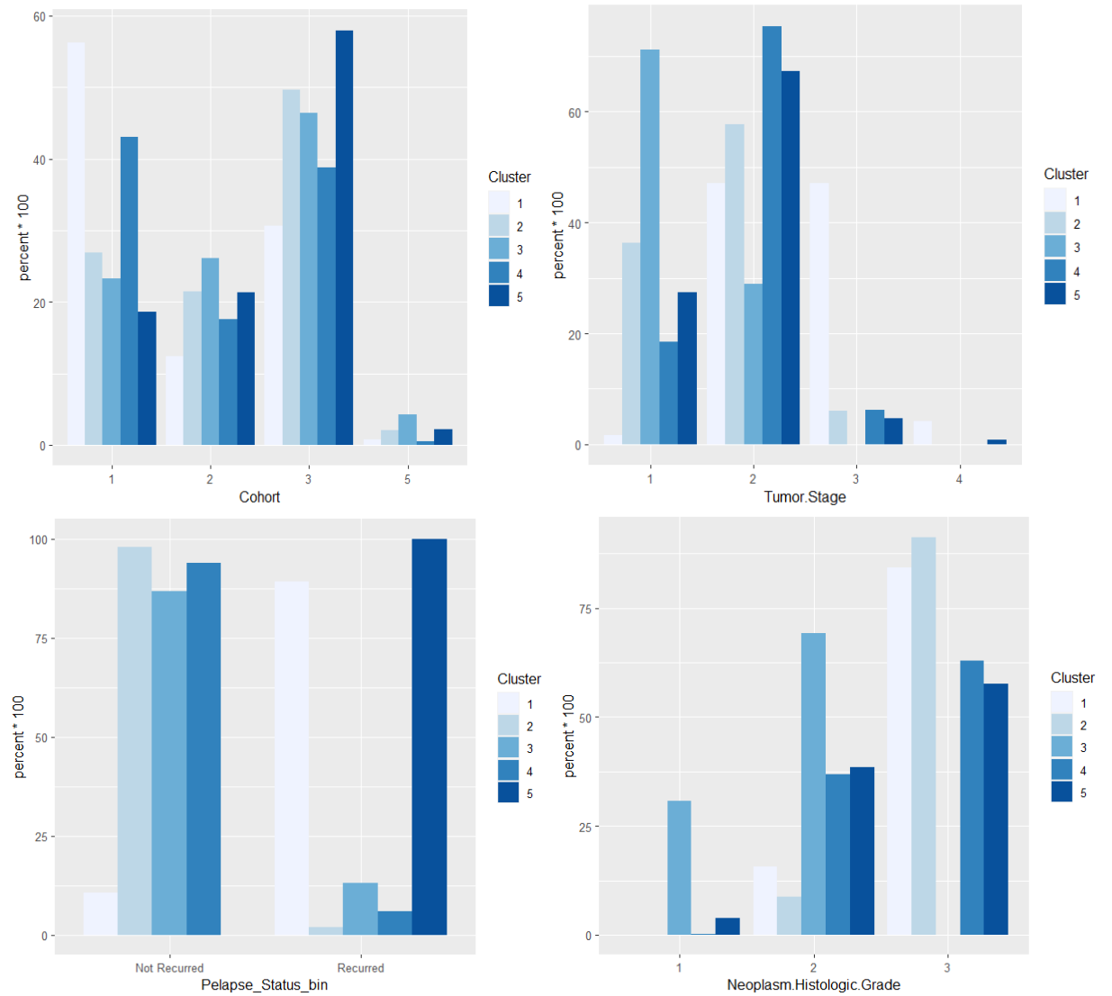
Picture 5 Categorical subgroup frequency group by 5 clusters
