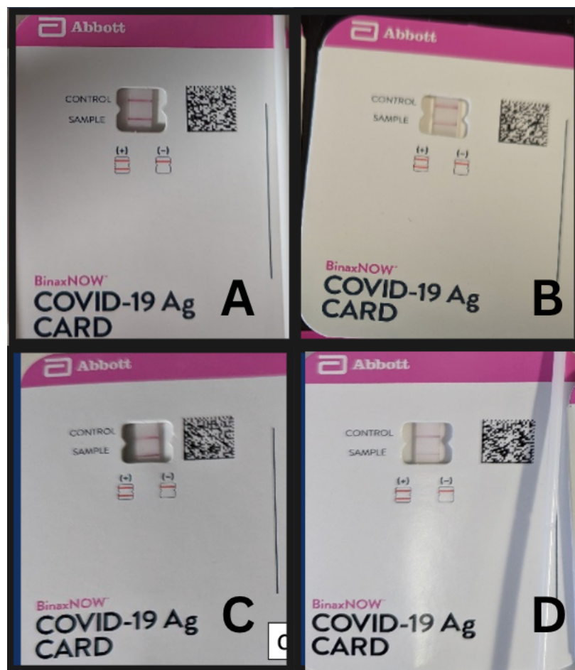
Figure 1: Unexpired and Expired Rapid Antigen Kits at varying viral concentrations
