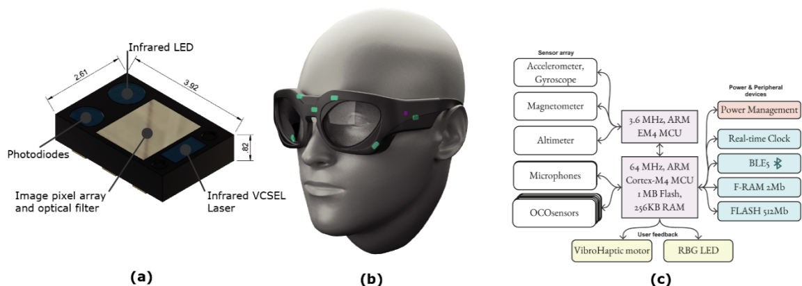
FIGURE 1. (a) shows a 3D render showing a future OCO™ sensor application specific integrated circuit (ASIC) and its dimensions and fundamental components. (b) shows a 3D-render of the OCO™ glasses on an average head model. The OCO™ sensors (green rectangles), and the IMU (purple rectangle) are highlighted on the model. (c) diagram showing the main electronics components within the OCOsense™ glasses.
