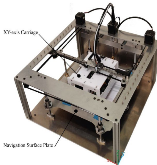
FIGURE 2. The computer numerical controlled (CNC) skin testing machine developed by Emteq that can move an OCO™ sensor development kit over human skin tissue samples in 3 dimensions. The sensors are mounted in the XY-axis carriage and can be moved in the X&Y-axis, the skin samples can be placed on the navigation surface plate and can then be moved in the Z-axis.
