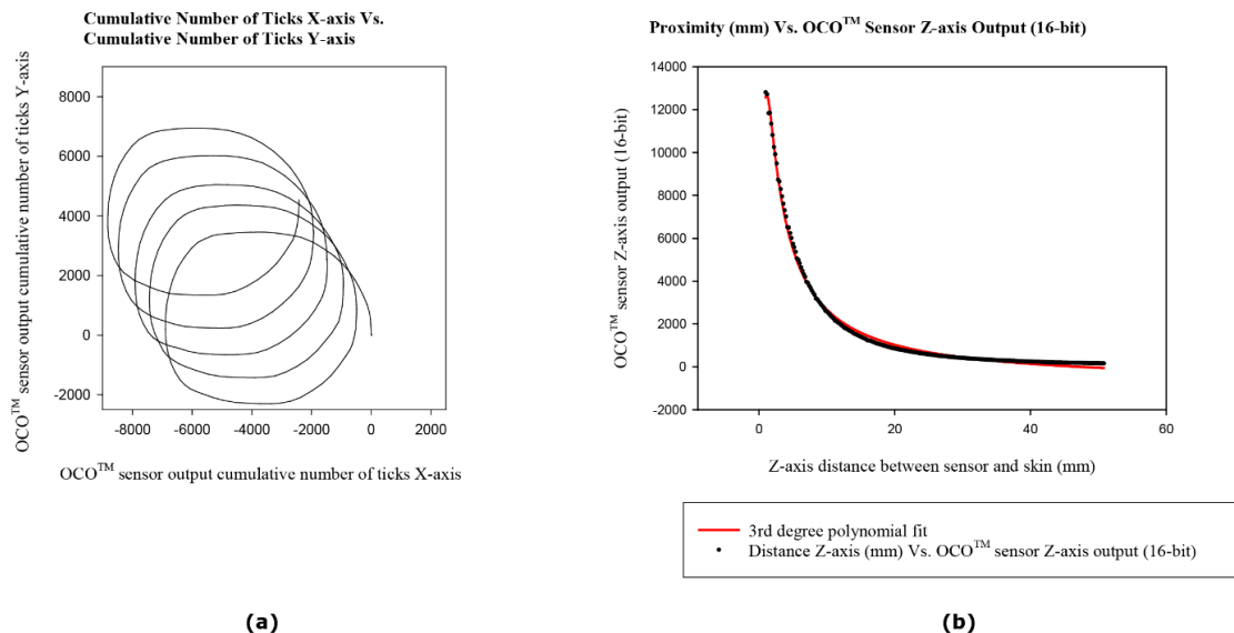
FIGURE 3. (a) is an example the OCO™ sensor’s X&Y-axis output data, the sensor was moved in a circular motion (15mm radius) over a human skin tissue sample at a velocity of 5,000mm/min at a constant proximity of 18mm, for 5 repetitions. (b) shows the OCO™ sensor’s Z-axis output data, the sensor was moved in the Z-axis from 4mm to 50mm away from the skin sample in 0.2mm increments.
