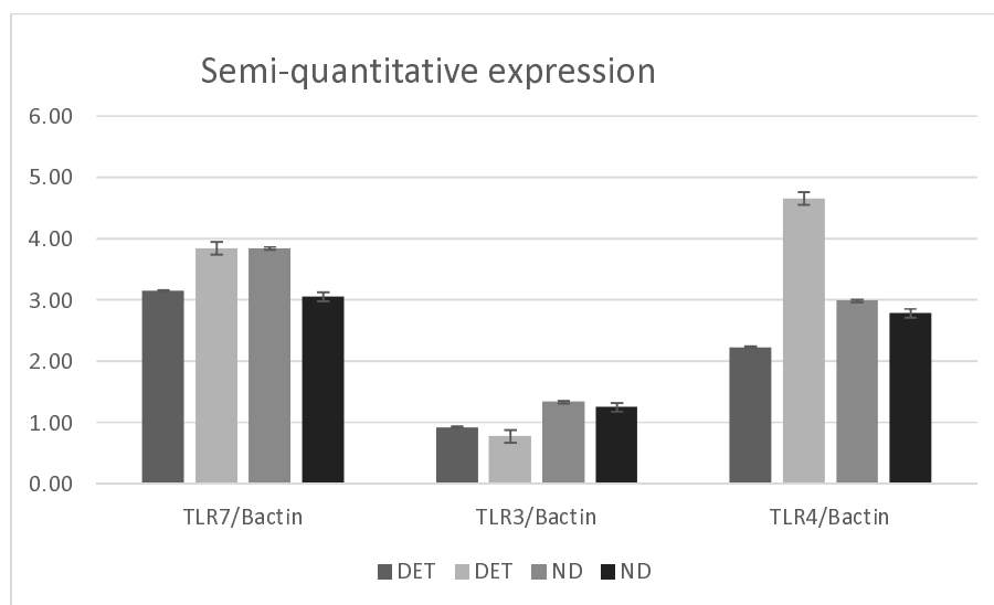
Histogram 2: TLRs expression in the 4 studied cohorts.
