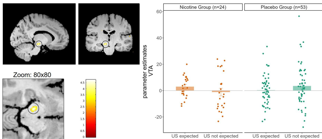
Figure 5. Stronger activation in the SN/VTA in the Nicotine group, when subjects expected the US, when compared to the Placebo group over the whole Fear Acquisition. Scatterpoints represent single subject contrast estimates in the SN/VTA, bars represent means with standard errors.
