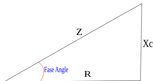
Figure 3: Relations between the components of bioimpedance.
