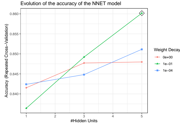
Figure 5: NNET model training.
