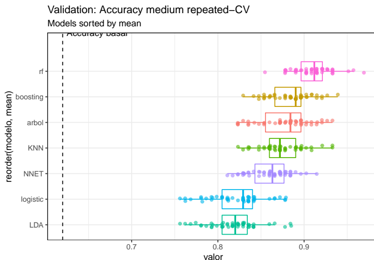
Figure 7: Boxplots of final model results.
