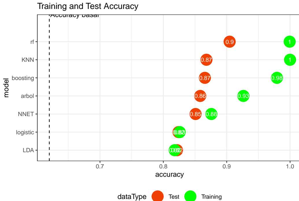
Figure 8: Results of applying the different models to the training and test data.
