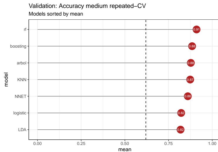
Figure 6: Final results of the training of the different models.
