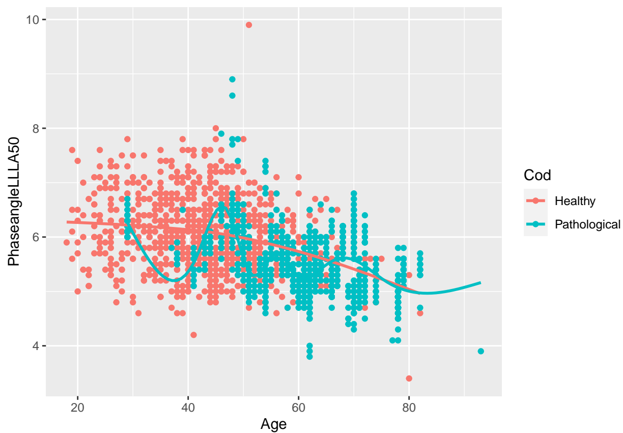
Figure 12: Graphical representation of the phase angle between left leg and left arm according to age in the different groups with frequencies of 50 kHz.
