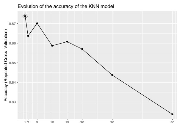
Figure 4: Graphical representation of the training KNN with the values de k used.
