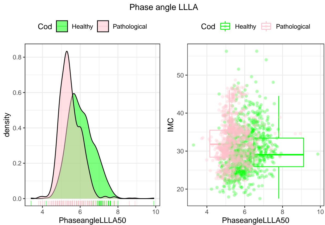
Figure 10: Density and IMC of the two groups based on the phase angle between the left leg and left arm with frequencies of 50 kHz.
