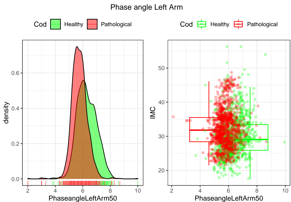
Figure 9: Density and IMC of the two groups based on the phase angle of the left arm with frequencies of 50 kHz.
