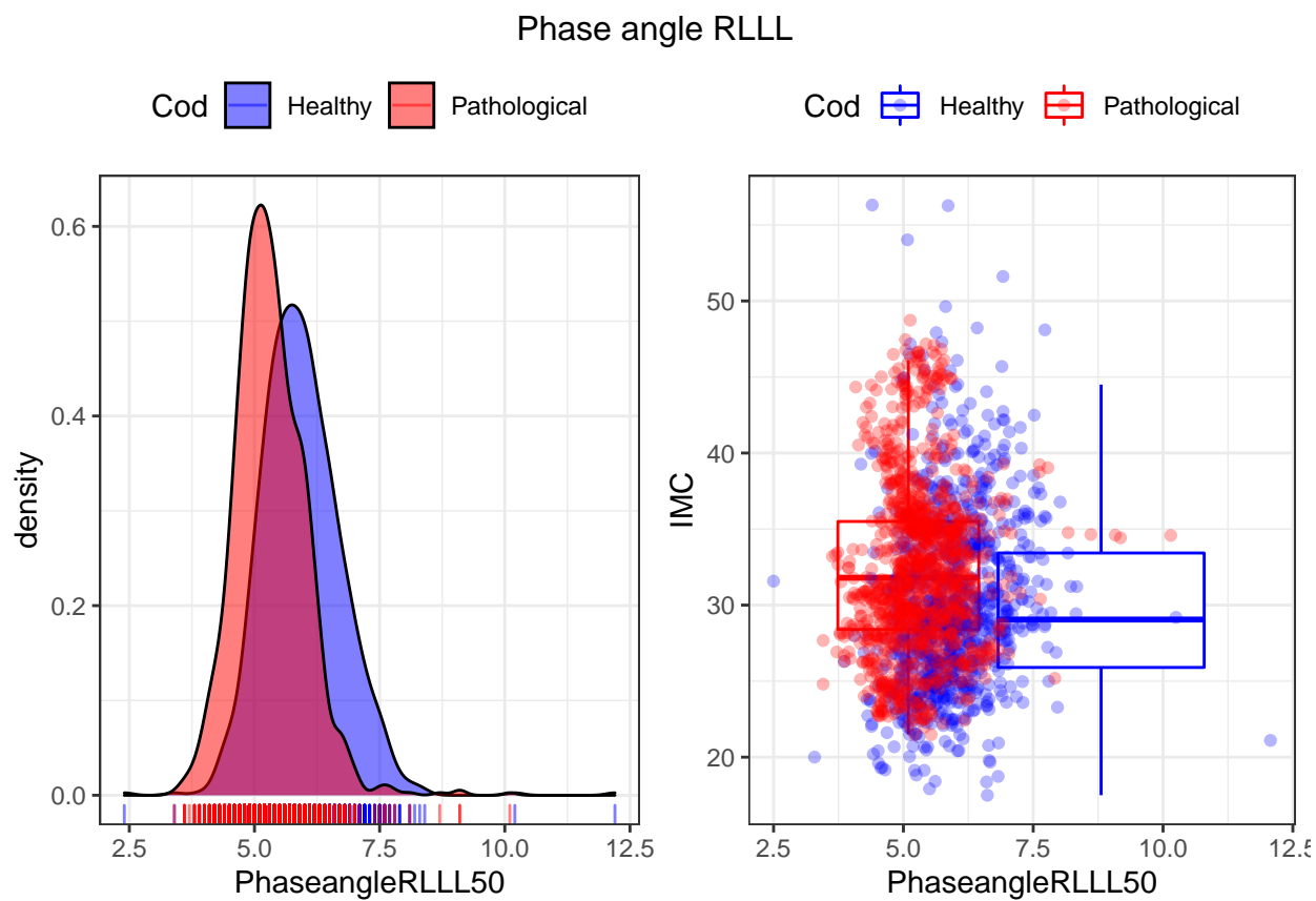
Figure 11: Density and IMC of the two groups based on the phase angle between the right leg and left leg with frequencies of 50 kHz.
