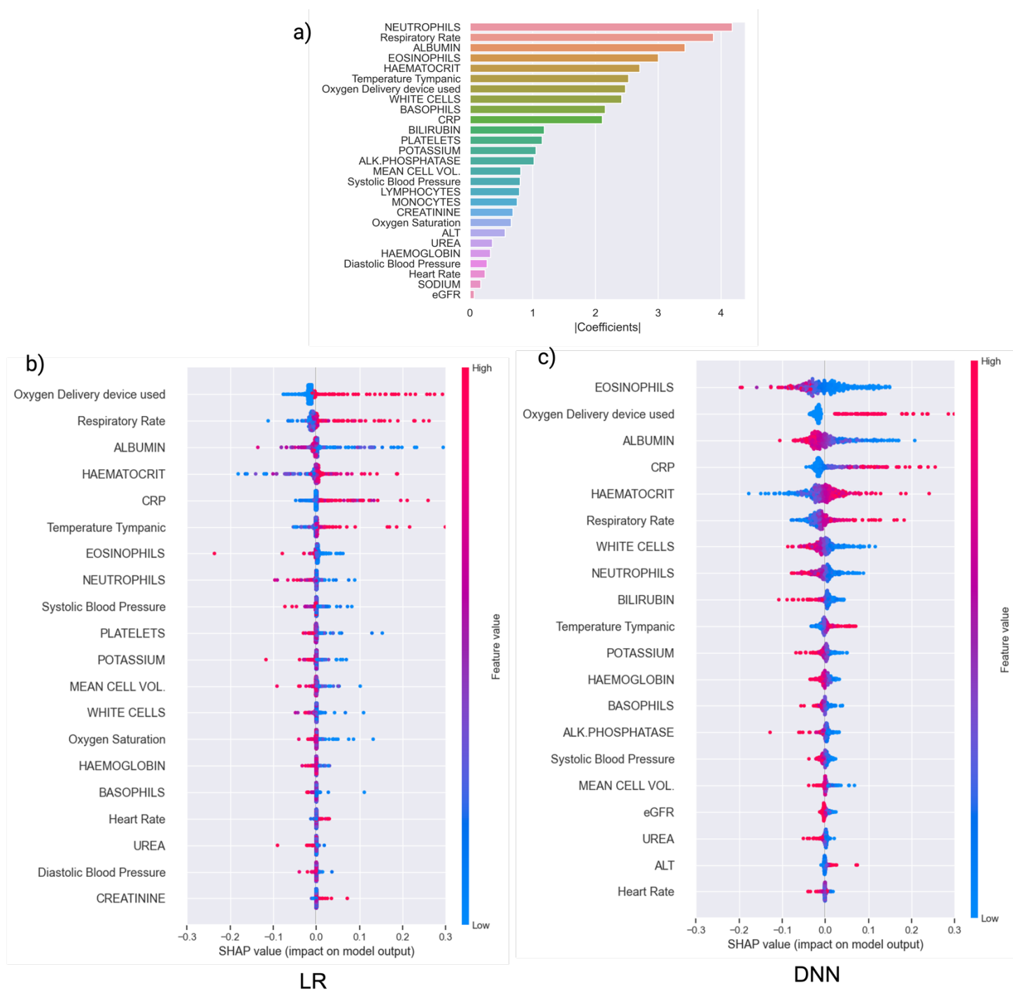
Figure 4: Explainability analyses. (a) logistic regression coefficient scalars within the final global model. (b) and (c) SHAP values for the 20 features with greatest impact on predictions made by the LR and DNN global models respectively, calculated during centralised external validation at BH and shown as beeswarm plots. Each dot represents a patient attending BH during the prospective evaluation period. Positive SHAP values indicate a change in the expected model prediction towards testing positive for COVID-19. Features are shown in descending order of mean absolute SHAP value, with most impactful features shown at the top.
