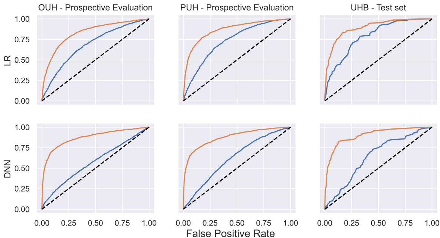
Figure 2: Receiver operating characteristic curves showing performance of (i) locally trained models prior to federation (blue), and (ii) the federated global model (orange) during prospective validation at OUH & PUH, and during evaluation on the locally-held test set at UHB. The area between receiver operating characteristic curves denotes the performance improvement on federation.
