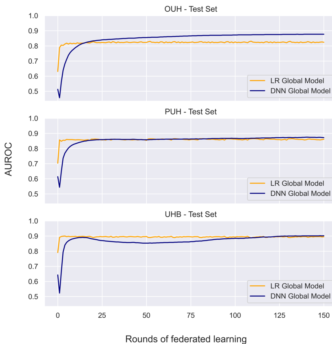
Supplementary Figure S2: Curves showing iterative improvement in performance (AUROC) of the global model after each round of federated training, evaluated on the held-out test set for each site participating in training.
